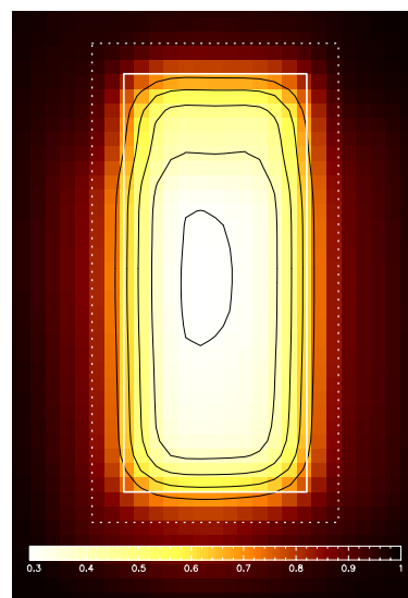
Fig. 12. Fourier optical prediction for how the total slit loss from a point source varies with its placement within a single shutter at a wavelength of \lambda = 2.0 \mu\text{m} . The shutter open area and pitch are indicated by the solid and dotted white lines.
