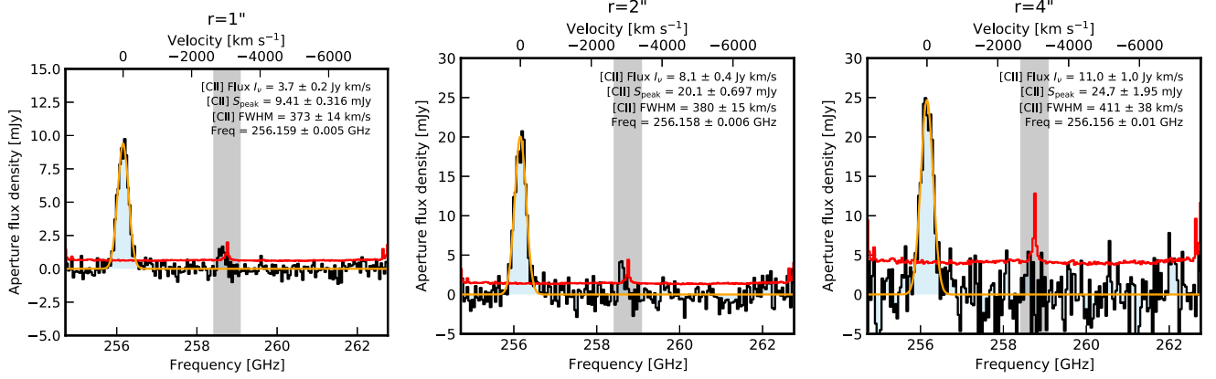
Figure 16. Continuum-subtracted aperture-integrated [C II] 158 \mu m spectra (black) for circular apertures with radii r = 1'' , 2'' , and 4'' . The best-fit Gaussian is shown in orange, and the best-fit parameters are displayed in the upper right corners of each plot.
