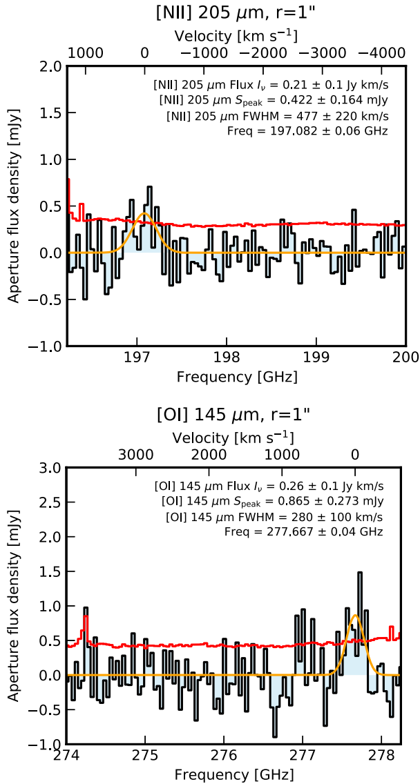
Figure 4. Continuum-subtracted spectrum of the [N II] _{205\,\mu\text{m}} (upper panel) and [O I] _{146\,\mu\text{m}} (lower panel). The spectra (black lines, shaded blue) are extracted in r = 1'' apertures centered on the peak of the emission in the velocity-integrated maps (Figure 3) using residual scaling (see Section 2). The 1\sigma noise level per channel for an r = 1'' aperture is shown in red, and a single-Gaussian fit is shown in orange (the best-fit parameters and uncertainties are in the upper right corners).
