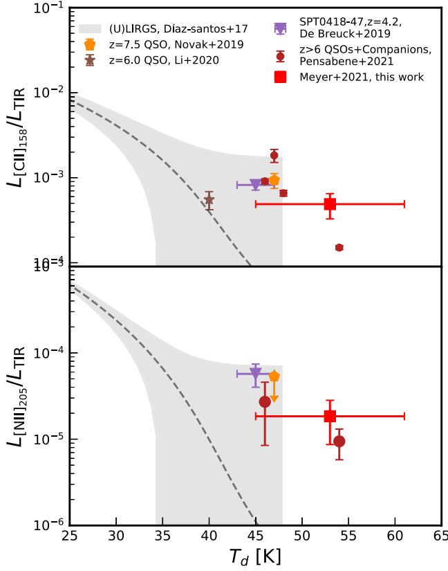
Figure 9. [C II]_{158 \mu m} and [N II]_{205 \mu m} line deficits of local (U)LIRGS (shaded gray; Díaz-Santos et al. 2017), the high-redshift galaxy SPT0418-47 (the purple triangle; De Breuck et al. 2019), and high-redshift quasars (the orange pentagon, dark orange star, and dark red circles; Novak et al. 2019; Li et al. 2020; Pensabene et al. 2021, respectively) and companion galaxies (the dark red circles; Pensabene et al. 2021). Our measurements for J1148+5251 are shown via the red squares.
