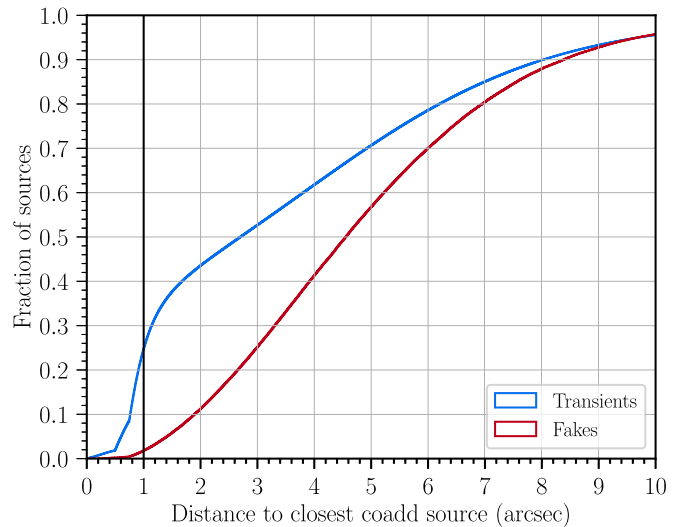
Figure 3. Cumulative histogram of the distance between each identified transient and the closest coadd source, measured for all putative transients (blue), and for the fake detections injected in the catalog (red). The blue curve shows a steep growth for distances \lesssim 1'' , while the fakes, which are uniformly distributed over the footprint, show much lower fractions with close coadds—24.3% (1.8%) of the transients (fakes) are closer than 1'' to a coadd source. This indicates that the close pairs are primarily associated with static sources, and not true solar system transients, so we remove them from the transient catalog.
