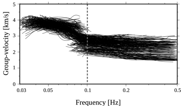
Figure 4. Measured dispersion curves for all possible inter-station paths (after removal of outliers). The dashed grey line separates the curves discarded (above 0.1 Hz) from the ones used in the tomography (below 0.1 Hz).
