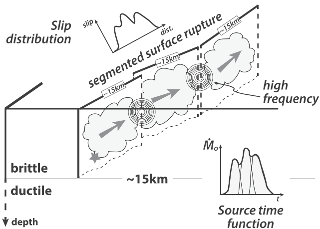
Figure 1. Schematic view of a strike-slip rupture including 3 sub-events. Interactions between nearby fault segments with different azimuth are generating additional high-frequencies. Independent evidence of consistent segmentation scaling are also found in surface-slip distribution, kinematic inversion results, source time function, and surface rupture geometry.
