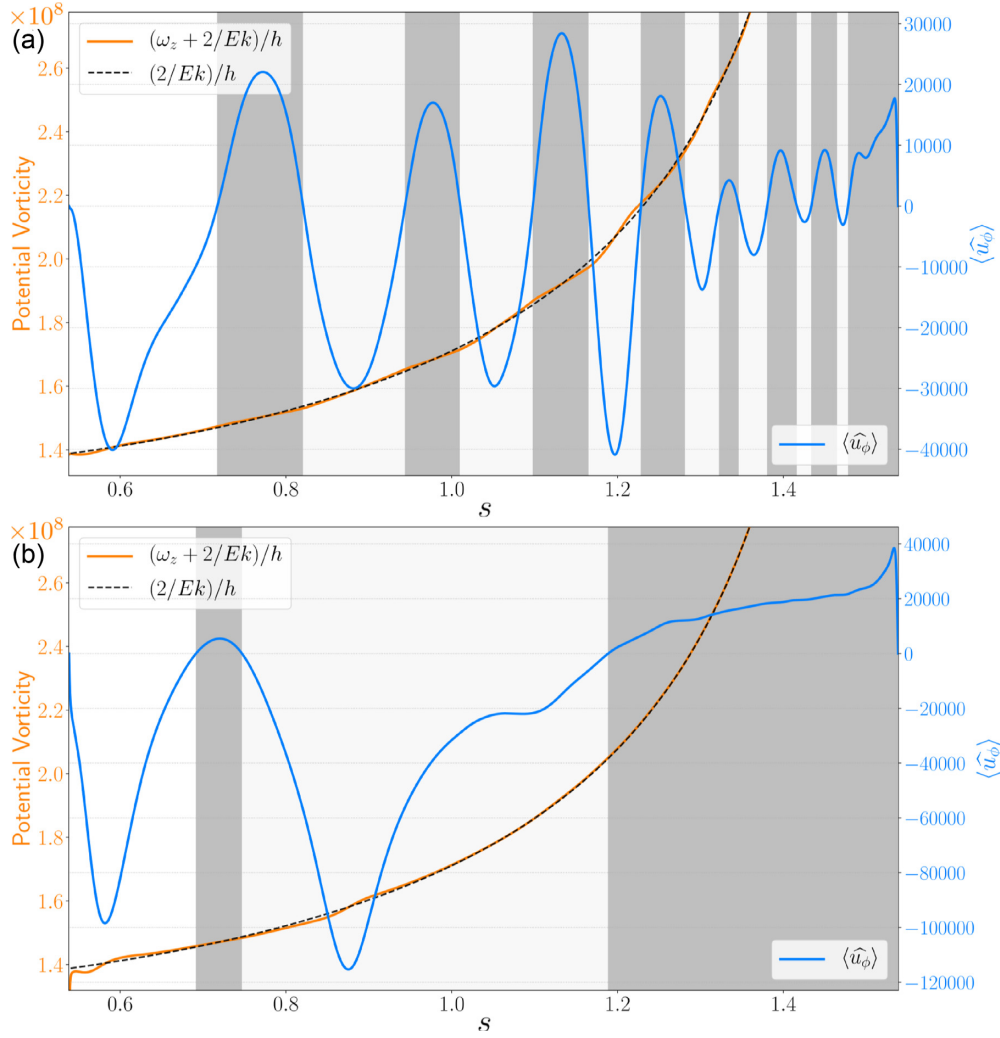
Figure 12. Time averaged radial profiles of the planetary vorticity 2Ek^{-1}/h (black-dotted curve), potential vorticity (\omega_z + 2/Ek)/h(s) (orange curve) and the azimuthal velocity \hat{u}_\phi(s) (blue curve); for the numerical simulation with parameters Ek = 10^{-8} , Pr = 1 , Ra = 8.99 \times 10^{12} = 142 Ra_c and a spatial resolution of (N_s, N_m) = (3073, 3072) (a), and the numerical simulation with parameters Ek = 10^{-8} , Pr = 10^{-2} , Ra = 3.37 \times 10^{10} = 6.1 Ra_c and a spatial resolution of (N_s, N_m) = (3457, 3456) (b). The shaded area and the white stripes correspond, respectively, to the fluid regions where the azimuthal velocity is positive (prograde jets) and negative (retrograde jets). The planetary vorticity (black-dotted curve) indicates the asymptotic behaviour of the potential vorticity in a perfectly mixed shell.
