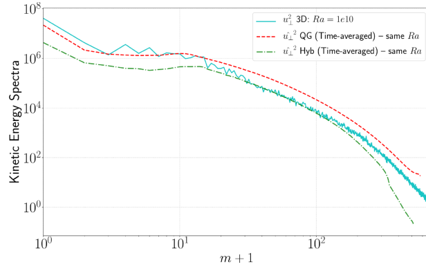
Figure 6. Kinetic energy spectra of the vertically averaged total velocity, \frac{1}{2}\mathbf{u}_{\perp}^2 = \frac{1}{2}(u_s^2 + u_{\phi}^2) , as a function of the order m + 1 , for the 3-D (cyan plain line), hybrid (green dotted–dashed line) and QG (orange dotted line) models, for a configuration conducted with the same parameters in the three cases Ek = 10^{-6} , Pr = 1 and Ra = 1 \times 10^{10} . The resolution in the 3-D, hybrid and QG cases is, respectively (N_r, \ell_{\max}) = (321, 682) , (N_s, N_m)/(N_r, \ell_{\max}) = (513, 512)/(513, 341) and (N_s, N_m) = (577, 576) .
