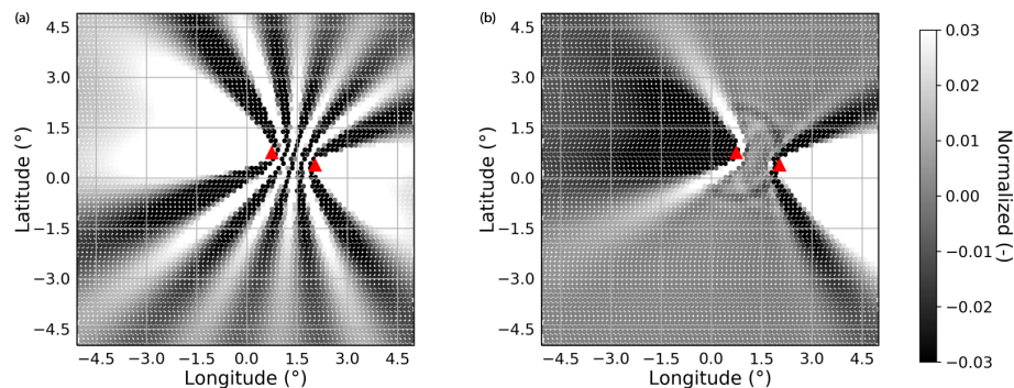
Figure 5. Illustration of sensitivity kernels. (a) Normalized vertical-component sensitivity kernel K_{zz}(\mathbf{x}_1, \mathbf{x}_2, \xi) of full waveform L2 misfit \chi_{\text{fwi}} (Eq. 9). The station locations \mathbf{x}_1, \mathbf{x}_2 are marked by red triangles. Frequency integration runs from 0 Hz to the Nyquist frequency, but the source spectrum peaks at dominant frequency 0.05 Hz and filters out everything above 0.1 Hz. (b) Normalized sensitivity kernel K_{zz}(\mathbf{x}_1, \mathbf{x}_2, \xi) of windowed asymmetry measurement \chi_A (Eq. 11). Similar figures can be obtained by adapting the Jupyter Notebook tutorial for noisi .
