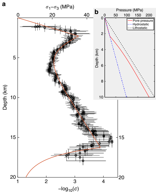
Fig. 4 Differential shear stress and the time delay before the onset of the power-law aftershock decay rate with respect to depth in California. a Logarithm of the most probable c -value for p = 1 with respect to the mean depth of the selected aftershocks within the 3 km depth bins (see all mainshocks in Fig. 2b). Error bars show the 95% Bayesian credibility regions for the c -value. The differential shear stress (red line) is derived from the Mohr–Coulomb theory using a coefficient of friction \mu = 0.75 , a porosity reduction mechanism at a depth of 2 km and a plastic flow law for wet quartzite (see “Methods” section and Table 1). b Evolution of pore (red), lithostatic (black), and hydrostatic pressures (blue) with respect to depth
