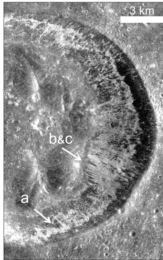
Figure 9. Bessel crater showing a portion of LRO Mini-RF instrument radar image (~30 m/pixel spatial resolution, image name LSR_CDR_LV00). Labels locate panels shown as close ups in LROC-NAC images in Figure 10. Image courtesy of NASA/GSFC/JHAPL.
