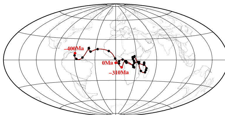
Figure B3. Location of the center of the African dome, for each 10 Myrs interval from –400Ma to present, in the paleomagnetic reference frame, superimposed to the present-day position of the continents (Hammer projection).
