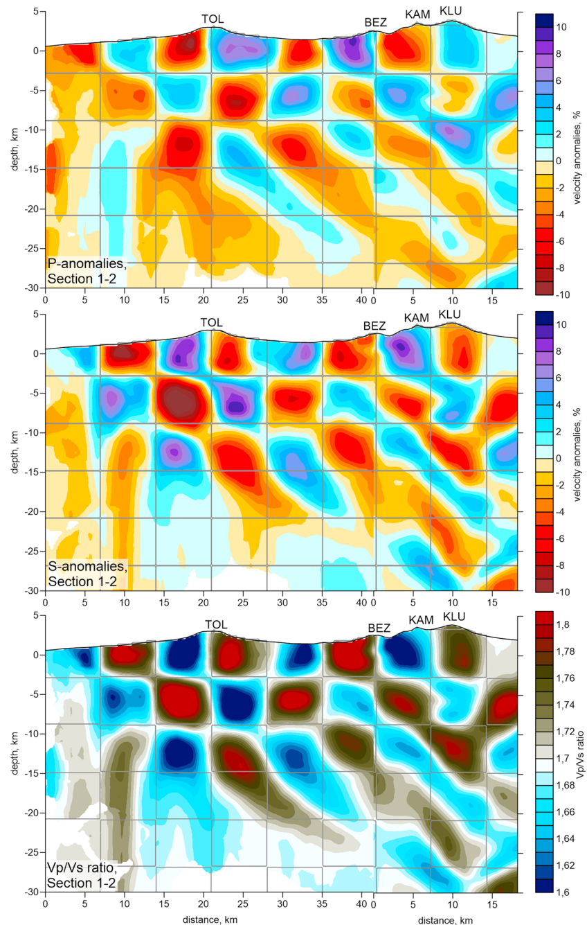
Figure 6. Recovery results for the P and S wave anomalies and the V_p/V_s ratios for the checkerboard model defined in sections 1 and 2 (see location in Figure 5). The configuration of the synthetic anomalies is highlighted with lines. Abbreviations are volcano names: TOL: Tolbachik, BEZ: Bezmianny, KAM: Kamen, KLU: Klyuchevskoy.
