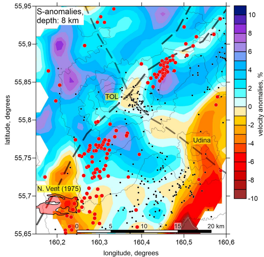
Figure 15. Horizontal section of the S wave velocity model at 8 km depth for the area of the Tolbachik volcano (TOL). The dotted lines indicate corrected locations of possible fault zones that cross beneath Tolbachik. The black dots denote seismic epicenters, and the red dots indicate monogenetic cones (as in Figure 1).
