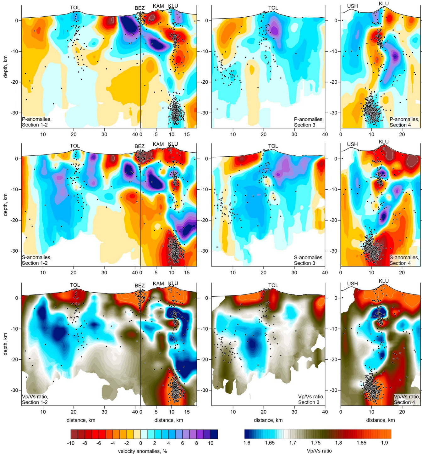
Figure 11. The resulting P and S wave velocities and Vp/Vs ratios in the vertical sections with locations indicated in Figures 8–10. The black dots denote earthquakes located within 3 km of the profile. The major volcanoes are indicated as follows: TOL: Tolbachik, BEZ: Bezmianny, KAM: Kamen, KLU: Klyuchevskoy, USH: Ushkovsky.
