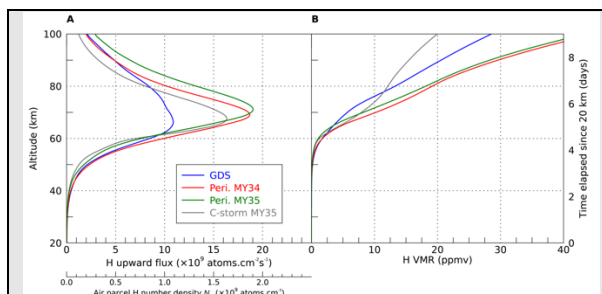
Figure 4: A synthesis of the four configurations explored with the air parcel model: MY34 GDS/Perihelion, and MY35 Perihelion/C-storm. (A) H Upward flux and concentration in the parcel during its rise from 20 to 100 km. (B) Same as (A) except NH is converted into H vmr (ppmv).
