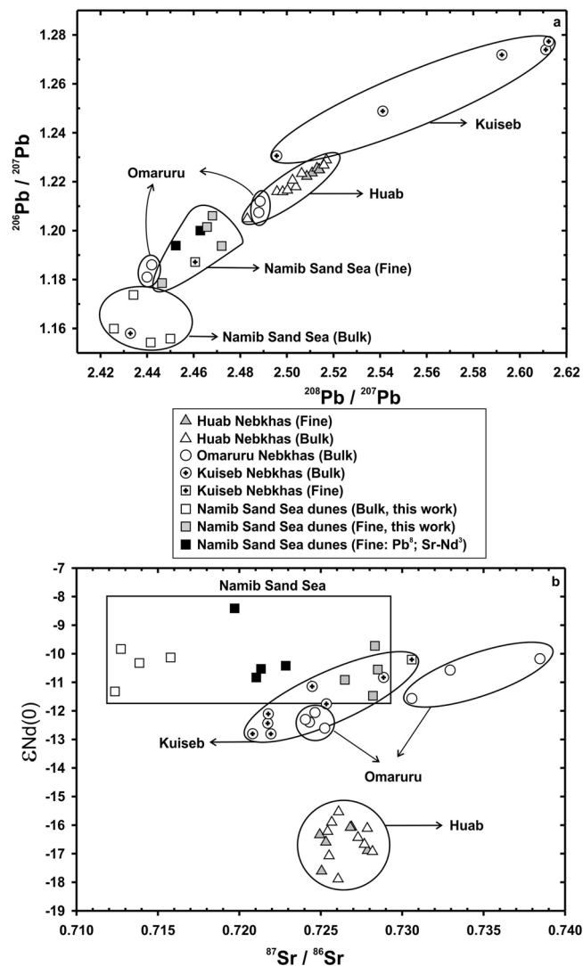
Fig. 3 Sr-Nd-Pb isotopic compositions of Southern Africa sediments. a ^{208}\text{Pb}/^{207}\text{Pb} vs. ^{206}\text{Pb}/^{207}\text{Pb} . b ^{87}\text{Sr}/^{86}\text{Sr} vs. \epsilon\text{Nd}(0) . Grain size effects on Sr-Nd-Pb isotopic compositions for the Huab and Namib Sand Sea are also shown and indicated by symbols in gray (fine) and open symbol (bulk).
