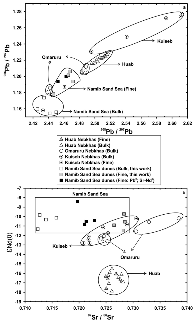
Fig. 3 Sr-Nd-Pb isotopic compositions of Southern Africa sediments.
