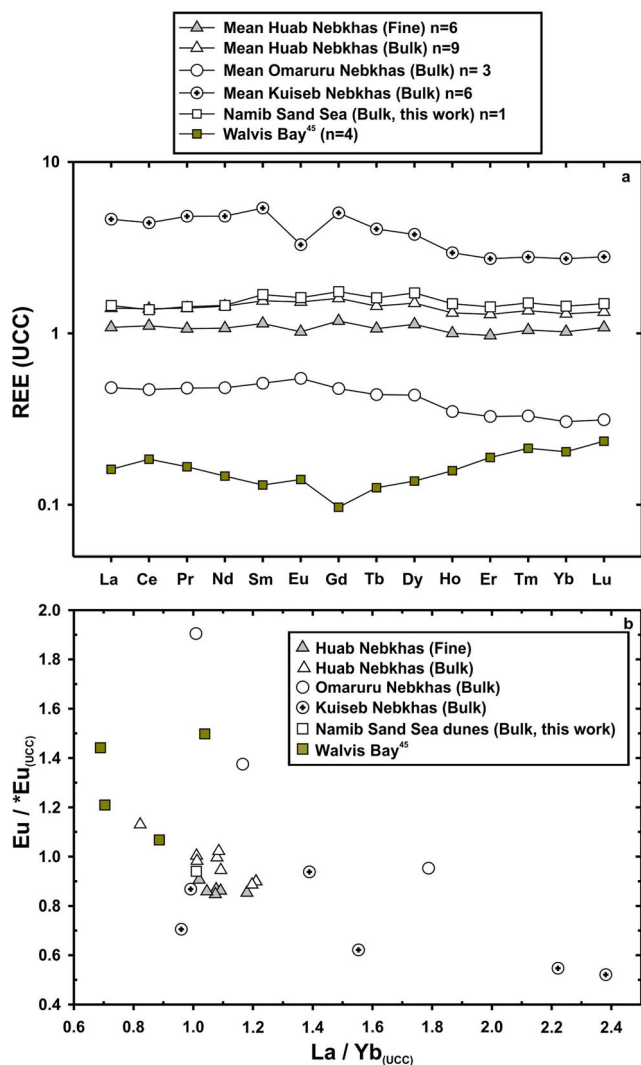
Fig. 2 Rare Earth Elements (REE) data of surface sediments representing the Potential source areas of Southern Africa. a Mean REE patterns. b Relationships between \text{Eu}/\text{Eu}^* and \text{La}/\text{Yb}_{\text{UCC}} . REE data has been normalized to upper continental crust 44 . Errors bars are smaller than symbols.
