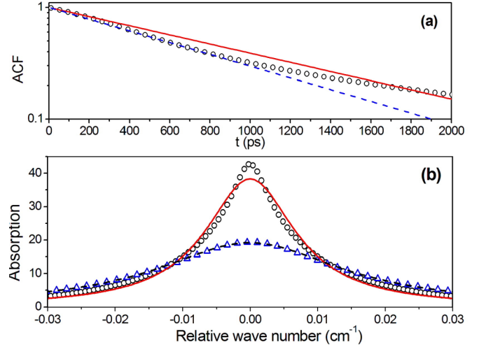
FIG. 6. (a) Dipole ACFs computed from Eq. (4) for \text{CO}_2 at 296 K, L = 0.2 \mu\text{m} , and \gamma P = 0 (black circles). The dashed blue line is the exponential decay giving the associated best fit and the full red line shows the results of Eq. (6). (b) Line shapes computed from Eqs. (4) and (5) (symbols) and corresponding Lorentzian fits (lines) for \text{CO}_2 at 296 K, L = 0.2 \mu\text{m} , \gamma = 0.1 \text{ cm}^{-1}/\text{atm} , and P = 0.02 \text{ atm} (black circles and full red line) and 0.1 atm (blue triangles and dashed black line).
