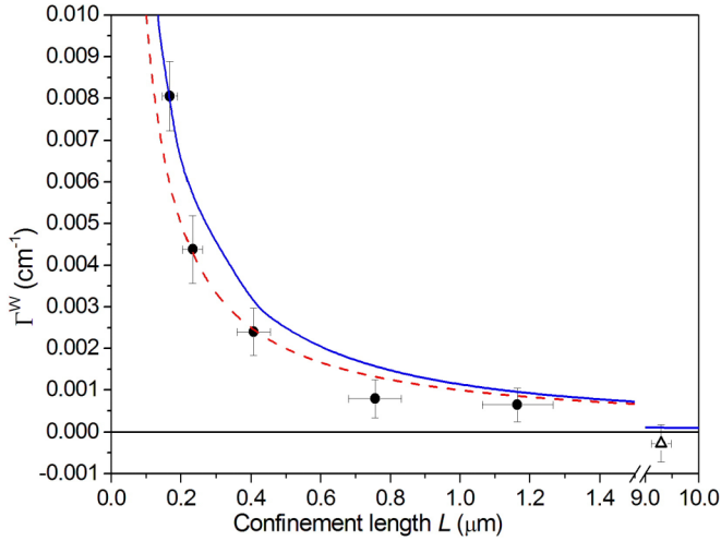
FIG. 5. Line widths (HWHMs) due to collisions of the \text{CO}_2 molecules with the cell windows as a function of the confinement length. The full circles are experimentally determined values from the present study while the open triangle was obtained from the measurements of [26]. The red dashed line gives predictions of Eq. (7) while the blue line was obtained from spectra computed using Eqs. (4) and (5) for the three measured pressures and treated as the experimental ones.
