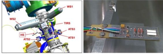
Figure 2. (Left) HS, WS, and ATS locations on the Remote Sensing Mast. (Right) HS without the cover; Humicaps®, which measure the relative humidity, are on right (white rectangles), Thermocap sensor heads next to them [1].
