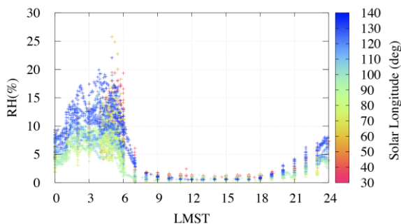
Fig. 2. Diurnal atmospheric relative humidity (%) for sols 65-275 (Ls ~ 36-134).
