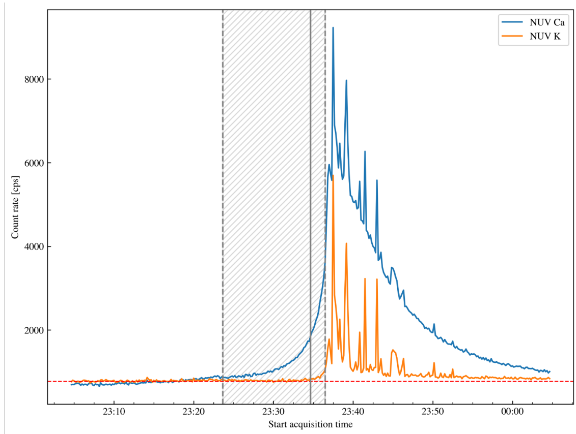
Fig. 2 c422 (blue) and c404 (orange) count rate as a function of time. The gray dashed area corresponds to BepiColombo being in the shadow of Mercury, the solid grey line represents the CA time and the red dotted line corresponds to the level of dark on c404 at the beginning of the observation.
