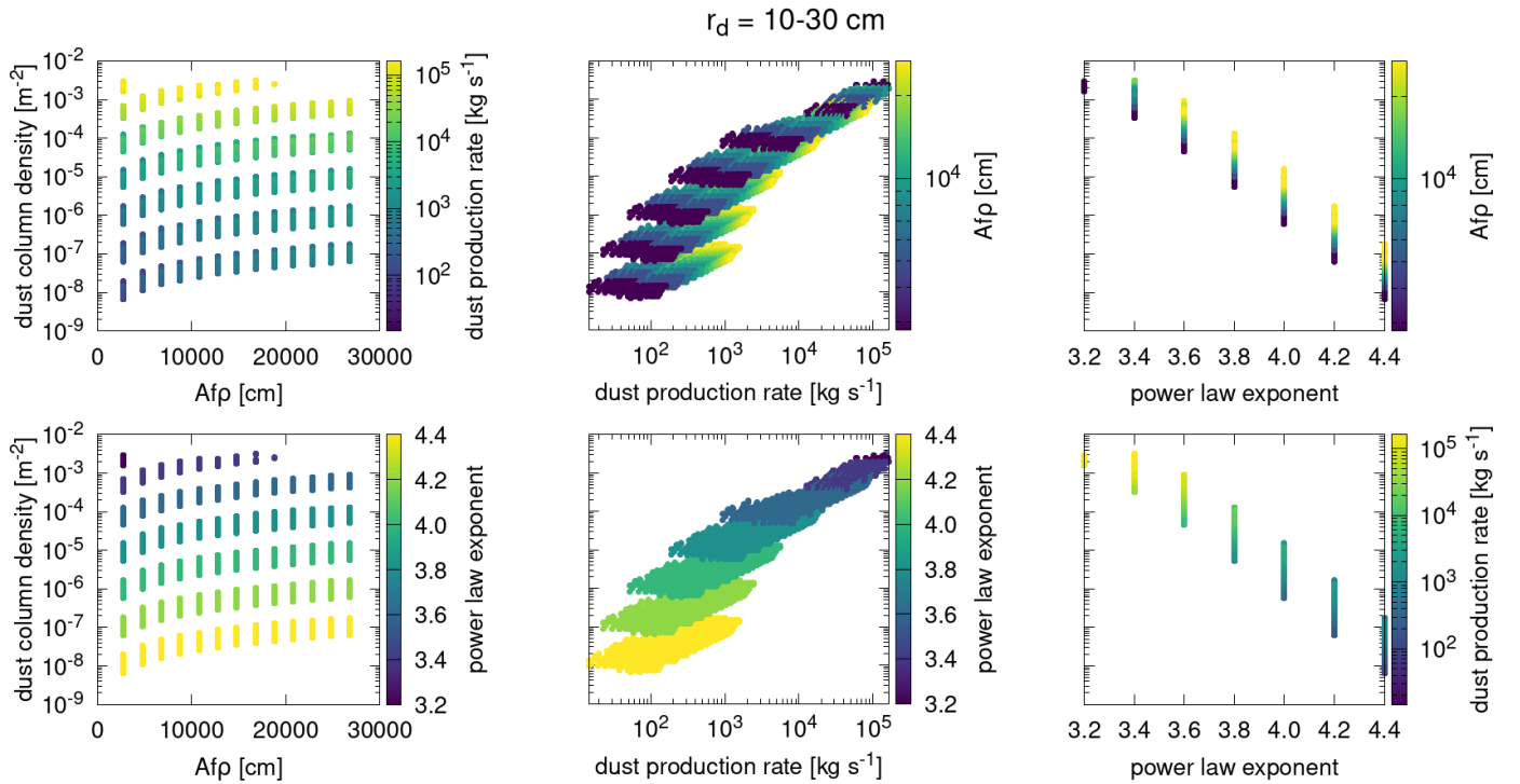
Fig. 9. Dust column density for dust particles with radii between 10 and 30 cm at the Comet Interceptor spacecraft A is shown as a function of different combinations of Af_p , the power law exponent, \beta , and the dust production rate.
