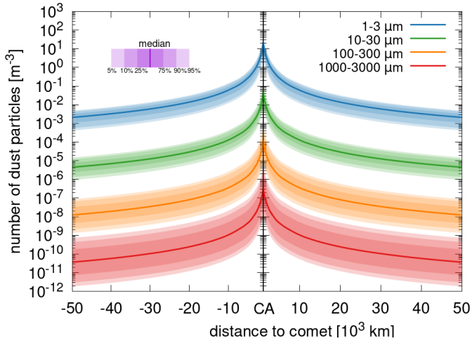
Fig. 6. Number of dust particles according to the EDCM along the spacecraft trajectory of spacecraft A as function of cometo-centric distance. The shaded areas show different percentile ranges within which cases fall. Closest approach for S/C A is assumed at 1000 km.
