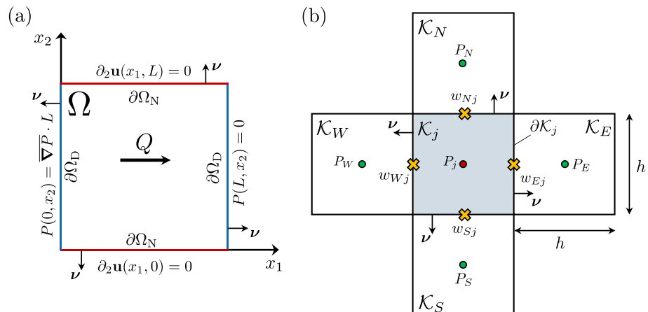
Figure 4. (a) Fracture plane representation with boundary conditions. (b) Finite volume method: five-point stencil. Pressures are defined at the center of each cell, while the fracture's local apertures are defined on the edges.
