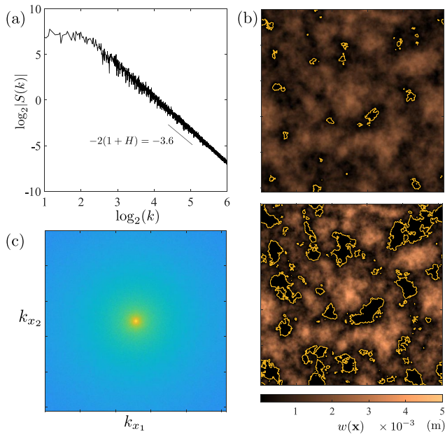
Figure 2. (a) Mean radial profile (obtained by angular integration) of the 2D Fourier transform of a fracture's aperture field, displaying a low-frequency cutoff for wave numbers smaller than k_c = 2\pi/L_c , and a power law (PL) trend of negative exponent -2(1+H) for higher frequencies. (b) Aperture field representations for different values of the closure: 0.5 (upper panel) and 1 (bottom panel). (c) Representation of the wave number to the power -(1+H) . The set of parameter adopted for the generations is L = 80 cm, L_c = 10 cm, \langle w \rangle = 1 mm, H = 0.8 .
