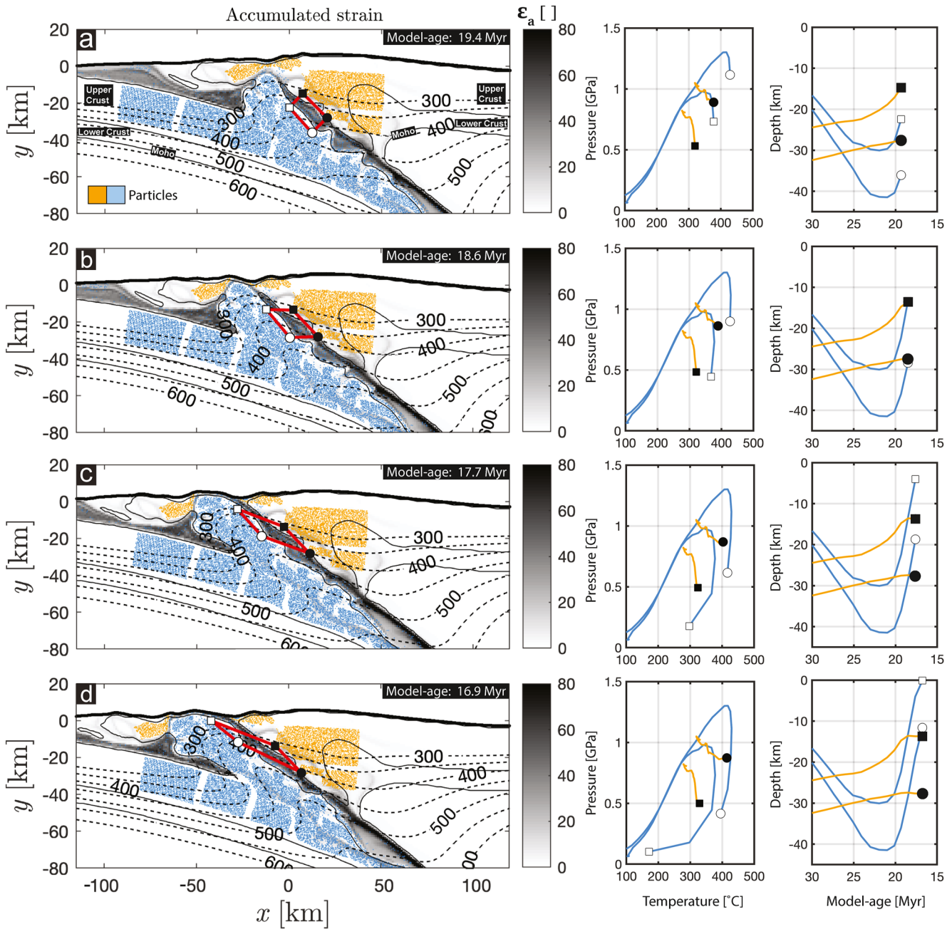
Figure 11. Evolution of accumulated strain ( \epsilon_a [ ]) is the time integral of the strain rate invariant at each numerical grid point and is dimensionless, where white colors indicate low strain and dark colors high strain) with pressure-temperature paths and depth-time paths for four selected markers that form the red parallelogram in the leftmost panels. Selected markers from overriding plate are yellow and markers from subducting plate are blue to visualize exhumation and lateral separation of upper plate during local extension. Dashed black lines indicate isotherms and numbers on dashed lines indicate temperature in ^{\circ}\text{C} . Rows (a–d) show results for four different model ages. Results are from the model with initially 6-km serpentinite thickness. The four corners of the red parallelogram are defined by markers whereby the two black markers are from the upper plate and the two white markers are from the subducting plate. The progressive shear deformation of the red parallelogram during exhumation indicates a normal-type shear sense between exhuming units and upper plate.
