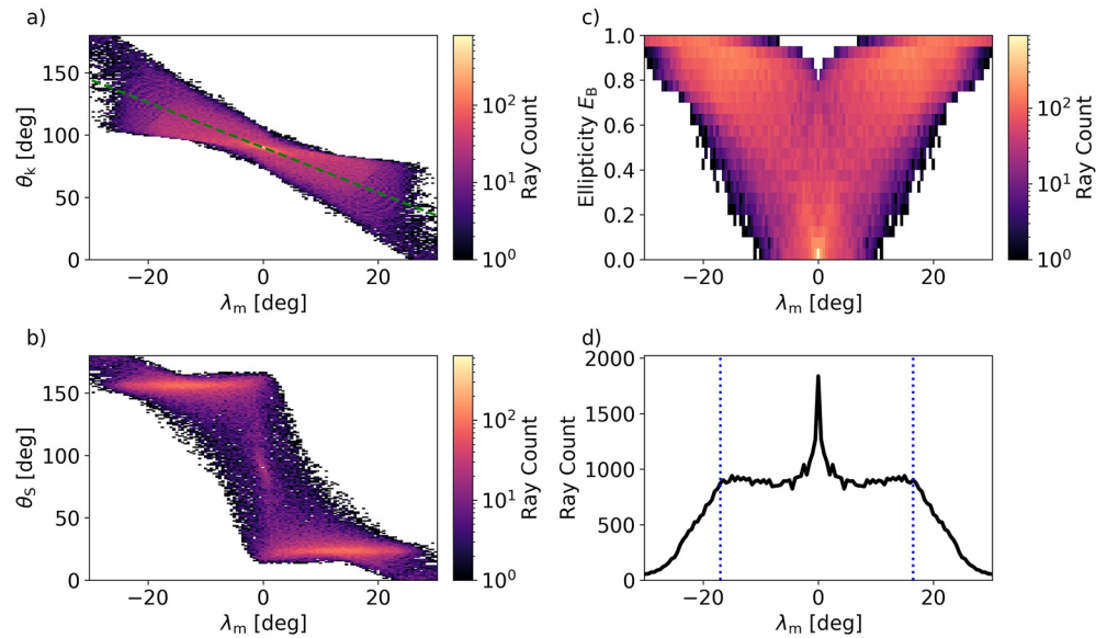
Figure 4. The same wave properties and distributions as in Figures 2a–2d, plotted as histograms of the number of simulated rays reaching low altitudes. The green dashed line in panel (a) is the linear least squares fit through all data points, with a slope of -1.81 . In panel (d) blue dotted lines give the \pm 17^\circ symmetric interval in which falls 75% of the rays.
