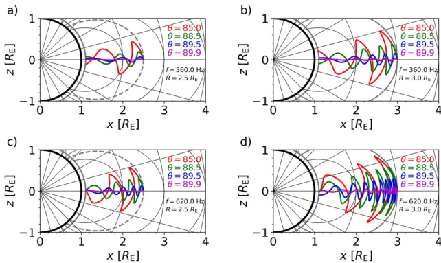
Figure 3. Propagation of selected rays with initial azimuthal angle \phi_{k0} = 180^\circ . The gray dashed line represents the initial L -shell of traced rays, the solid gray arc marks the orbital altitude of DEMETER. Thin black lines represent radial distances (with a step of 1 R_E ), latitudes (with a step of 15^\circ ) and L -shells (integer values). Individual ray trajectories are color-coded by their initial wave normal angle. Wave frequency and initial radial distance are given in each panel. The propagation times for these cases range from 2 to 8 s – see the Figure S2 in Supporting Information S1 for additional plots.
