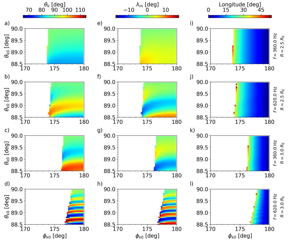
Figure 7. (a–d) Wave normal angles of simulated rays after reaching the altitude of DEMETER, plotted as a function of the initial wave normal angle \theta_{k0} and the initial azimuthal angle \phi_{k0} . (e–h) Latitude where rays crossed the altitude of DEMETER, same plot format as in (a–d). (i–l) Longitude where rays crossed the altitude of DEMETER, same plot format as in (a–d). On the right side of the figure, initial radial distances and wave frequencies are indicated for each triplet of plots.
