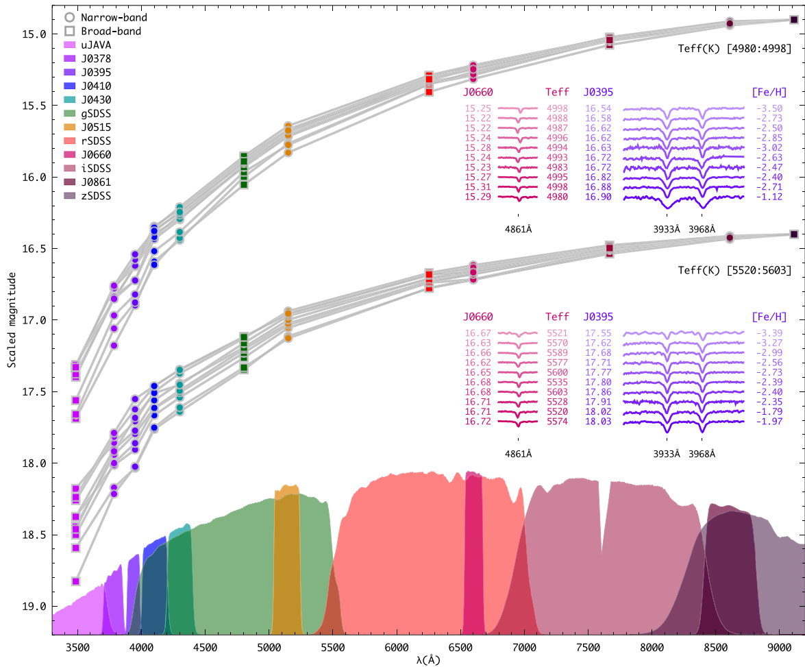
Figure 6. Spectral energy distribution (SED) for 20 selected program stars from Blanco and Gemini. Magnitudes were scaled to z\text{SDSS} = 14.9 (top) and 16.4 (bottom). The temperature range for each set is displayed right below the SEDs. The insets show the observed spectra around the H\beta and \text{Ca II HK} absorption features, sorted by their J0395 scaled magnitude. Also shown are the T_{\text{eff}} and [\text{Fe}/\text{H}] for each star and the S-PLUS transmission curves. See the text for further details.
