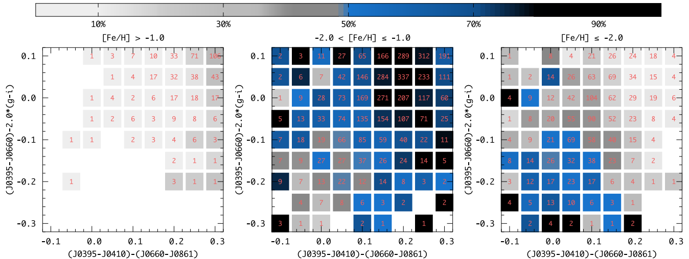
Figure 2. Color–color diagram for three different [Fe/H] regimes. The bins in each panel are color-coded by the fraction of stars with an average metallicity in a given range. The number of stars in each bin is also shown.
