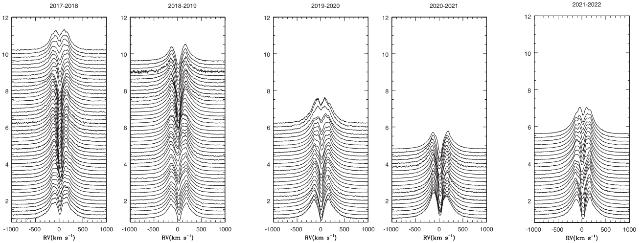
Figure A1. Evolution of the profile of the H\alpha line in the spectrum of HD 37202 over the latest five observing seasons. Time is running downwards.
