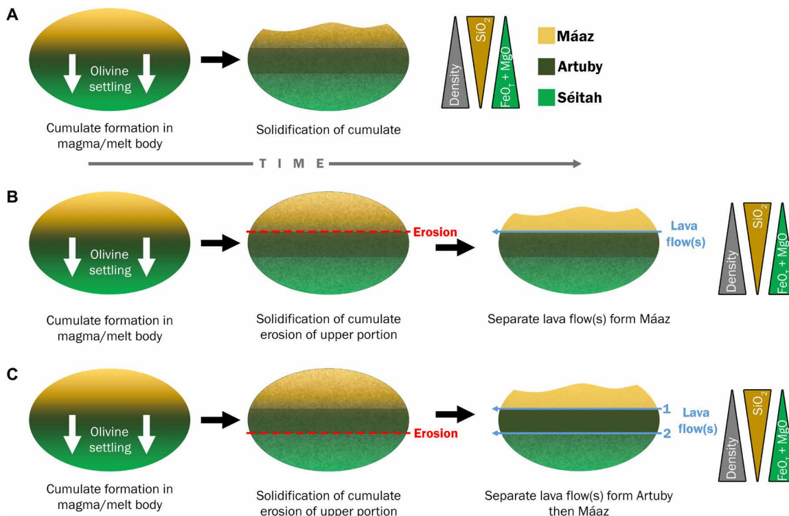
Fig. 8. Formation scenarios. (A) Cumulate formed from stratification of a single melt in which olivine phenocrysts were segregated by gravity in a magma body, which subsequently solidified. All of the rocks observed by SuperCam were produced within this igneous body in this scenario. (B) Cumulate plus lava flow(s) scenario, initiated with the fm of Séítah and Artuby as a cumulate as in (A). The depleted upper portions of the body were removed and subsequent lava flow(s) produced Máaz. (C) Third scenario in which Artuby was also produced by a relatively viscous lava flow before emplacement of Máaz by later and more evolved lava. Triangles at the right indicate overall composition and density trends.
