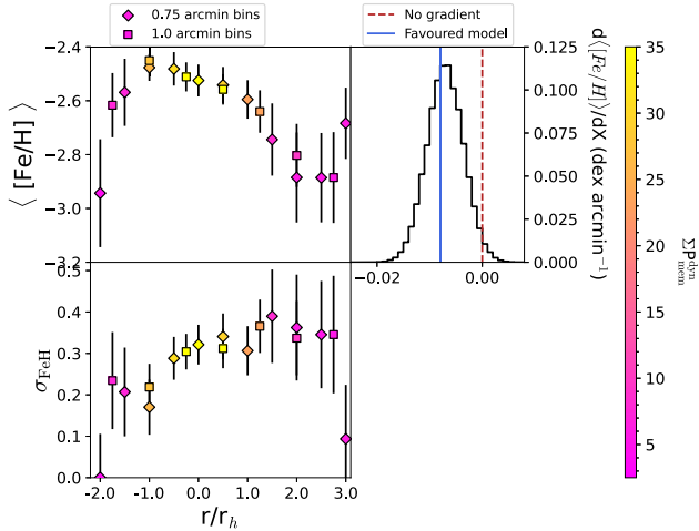
Figure 13. Similar plot as Fig. 9 for the metallicity model and metallicity dispersion.
