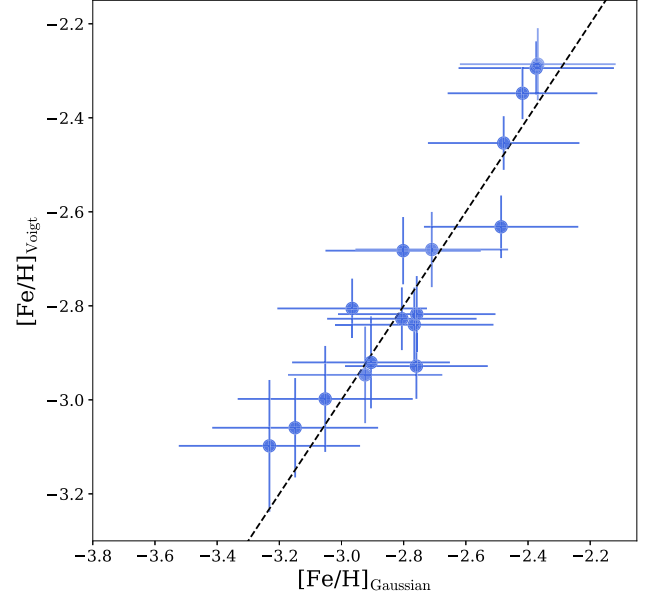
Figure 11. Comparison between the spectroscopic metallicities obtained with Gaussian line profiles and the S10 calibration on the x -axis and Voigt line profiles and the C13 calibration on the y -axis. The circles' opacity represent the dynamical membership probability of each star.
