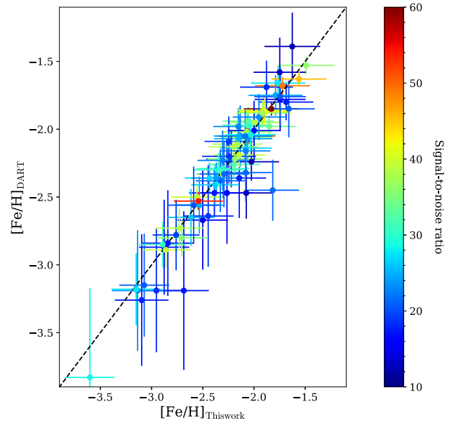
Figure 5. Comparison between the metallicities obtained with our new pipeline on the x-axis with the ones from the DART survey on the y-axis for a sample of 86 Sextans stars. The data are colour-coded according to their S/N ratios and the black dashed line shows the 1:1 line.
