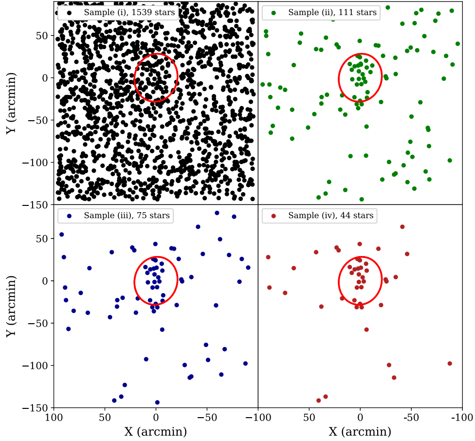
Figure 14. Spatial distributions of stars in the Boo I field for the four samples detailed in Section 3: only photometry (top left), photometry + Gaia (top right), photometry + Gaia + [\text{Fe}/\text{H}]_{\text{Pristine}} < -1.0 (bottom left) and photometry + Gaia + [\text{Fe}/\text{H}]_{\text{Pristine}} < -2.0 (bottom right). The two half-light radii of Boo I as derived by M18 are shown as the red ellipses.
