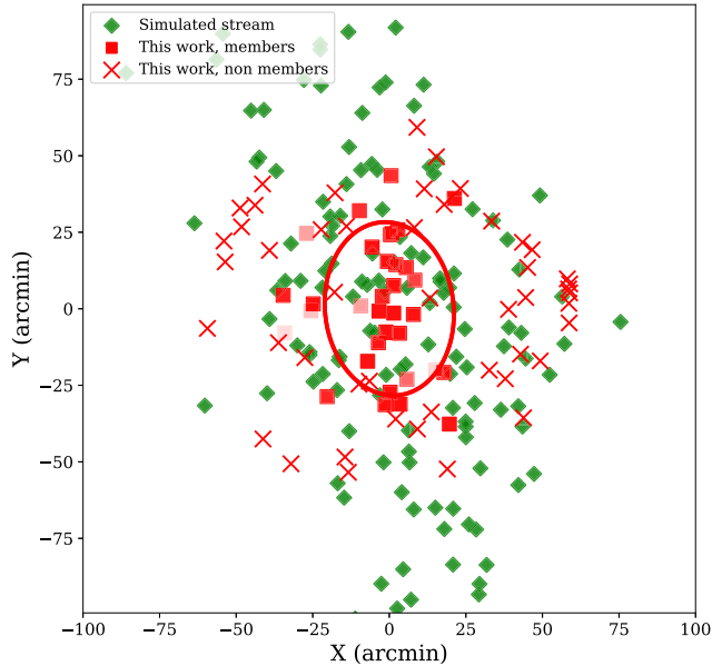
Figure 16. Spatial distribution of test particles in the hypothesis that Boo I is tidal disrupting (green diamonds) obtained with our toy model described in Section 3.3. The spectroscopic sample presented in this work is shown in red crosses (non-members) and squares (members). The two half-light radii of Boo I as derived by M18 are shown with the red ellipse.
