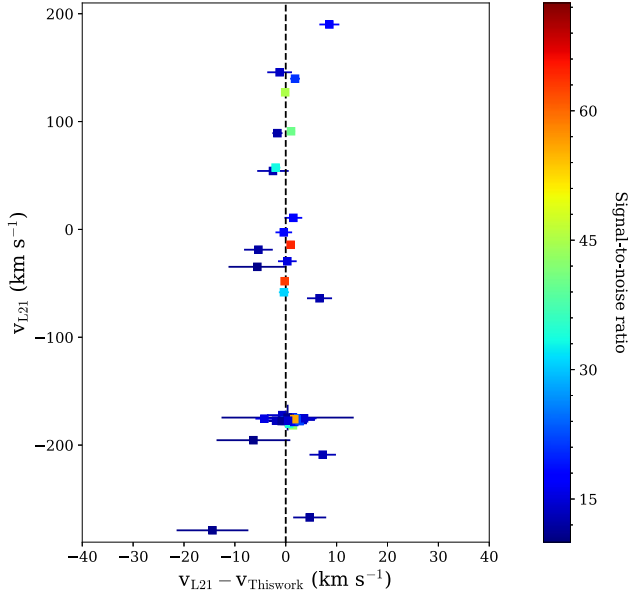
Figure 3. Difference between the radial velocities obtained with our new pipeline and the ones from L21 on the x-axis with respect the L21 velocities on the y-axis. The data are colour-coded according to their S/N ratios and the black dashed line shows the 0 \text{ km s}^{-1} offset line.
