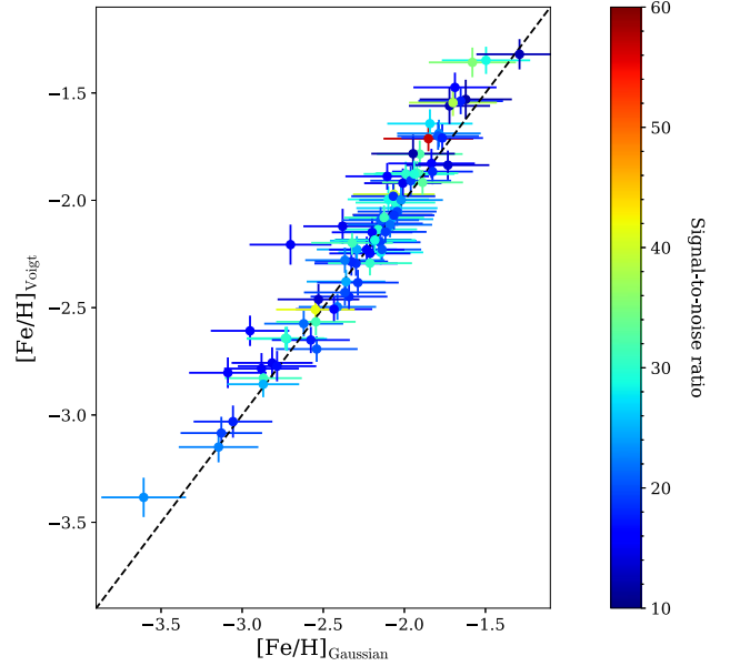
Figure 6. Comparison between the metallicities obtained with our new pipeline with Gaussian line profiles on the x-axis and with Voigt profiles on the y-axis for the sample of Sextans stars. The data are colour-coded according to their S/N ratios and the black dashed line shows the 1:1 line.
