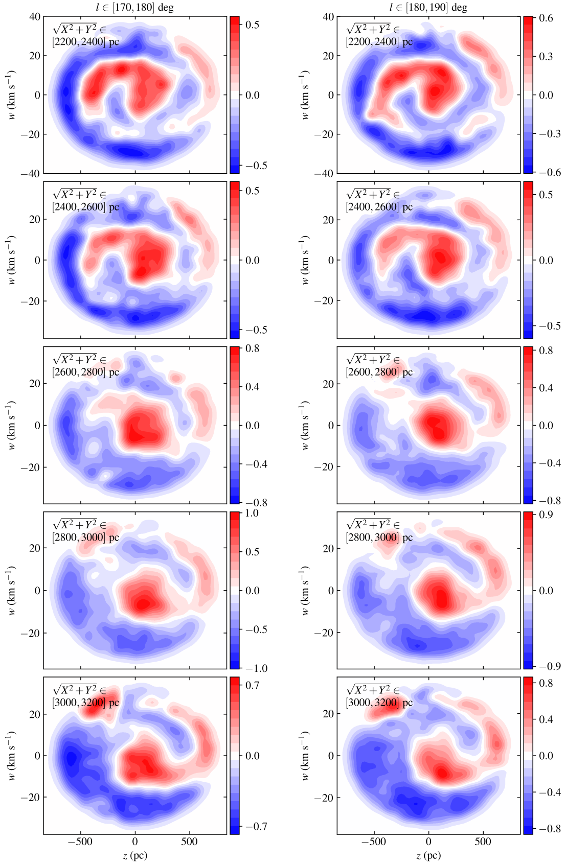
Fig. 6. Phase-space spiral seen in the direction of the Galactic anti-centre, for data samples with l \in [170, 180] degrees ( left column ) and l \in [180, 190] degrees ( right column ), and \sqrt{X^2 + Y^2} in range 2200–3200 pc (increasing from top to bottom ). The respective panels show the relative difference between the data histogram and fitted bulk density distribution: M \times (d - B)/B . The horizontal axis is identical for all panels.
