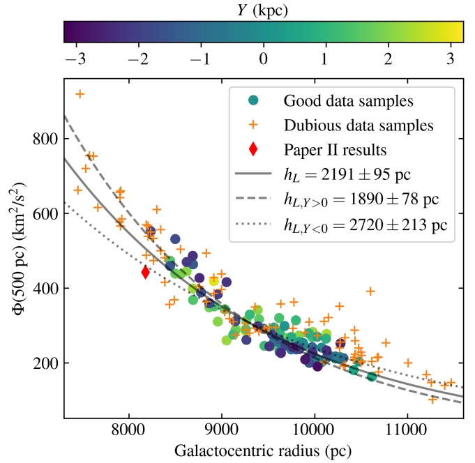
Fig. 10. Same as Fig. 9, but for |z| = 500 pc.
