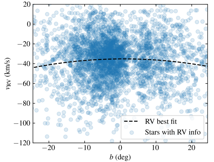
Fig. 2. Radial velocity ( v_{RV} ) as a function of Galactic latitude ( b ) for the data sample with l \in [90, 100] deg and \sqrt{X^2 + Y^2} \in [2200, 2400] pc. The dashed line corresponds to the fitted function and the scatter point correspond to stars with available radial velocity information. The range in b on the horizontal axis corresponds to a range in height spanning roughly Z \in [-1, 1] kpc at the relevant distance.
