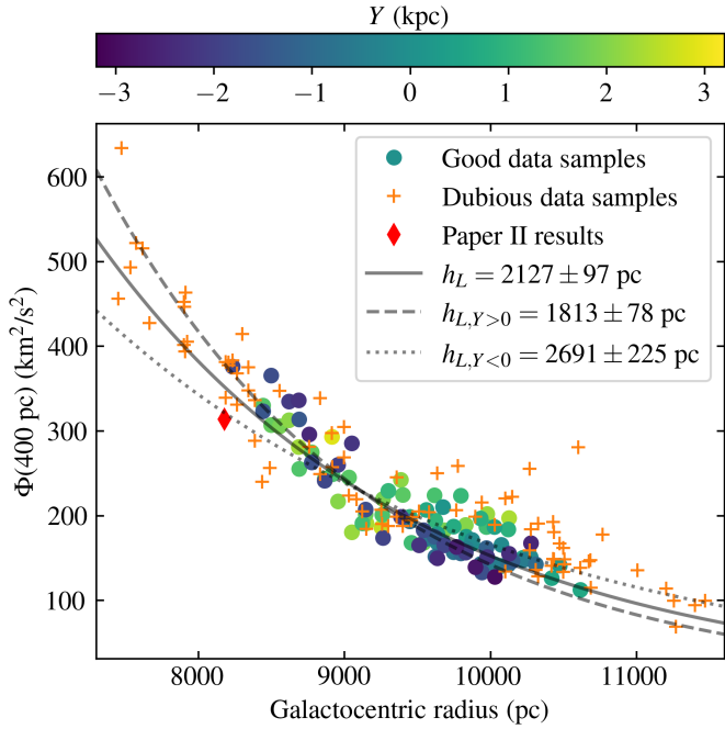
Fig. 9. Inferred gravitational potential at a height of |z| = 400 pc, as a function of Galactocentric radius. The results of the good data samples are marked with circles, which are colour coded according to the data samples’ respective Y coordinate. The dashed line shows a best fit exponential curve with respect to the good data samples. We also show the results coming from the dubious data samples, and the result of Paper II for the immediate solar neighbourhood.
