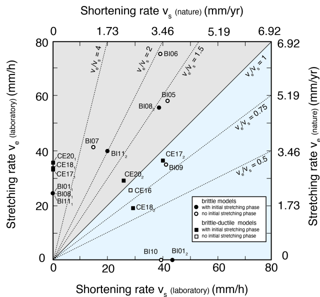
Figure 3. Applied boundary kinematic conditions for models with brittle crust (circles) and brittle–ductile crust (squares). Models with two-stage deformation have black filled symbols and subscripts to indicate the stage of deformation. Laboratory and scaled values are given for the shortening and stretching rates.
