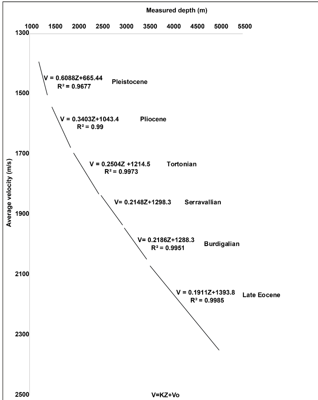
Fig. 4. A plot of average velocity ( V_{avg.} ) from checkshot data versus measured depth (m) in the deep FM 1 well (location in Figs. 1, 2), used in time-depth conversion of the seismically-defined surfaces (modified from Chima et al. 2022).
