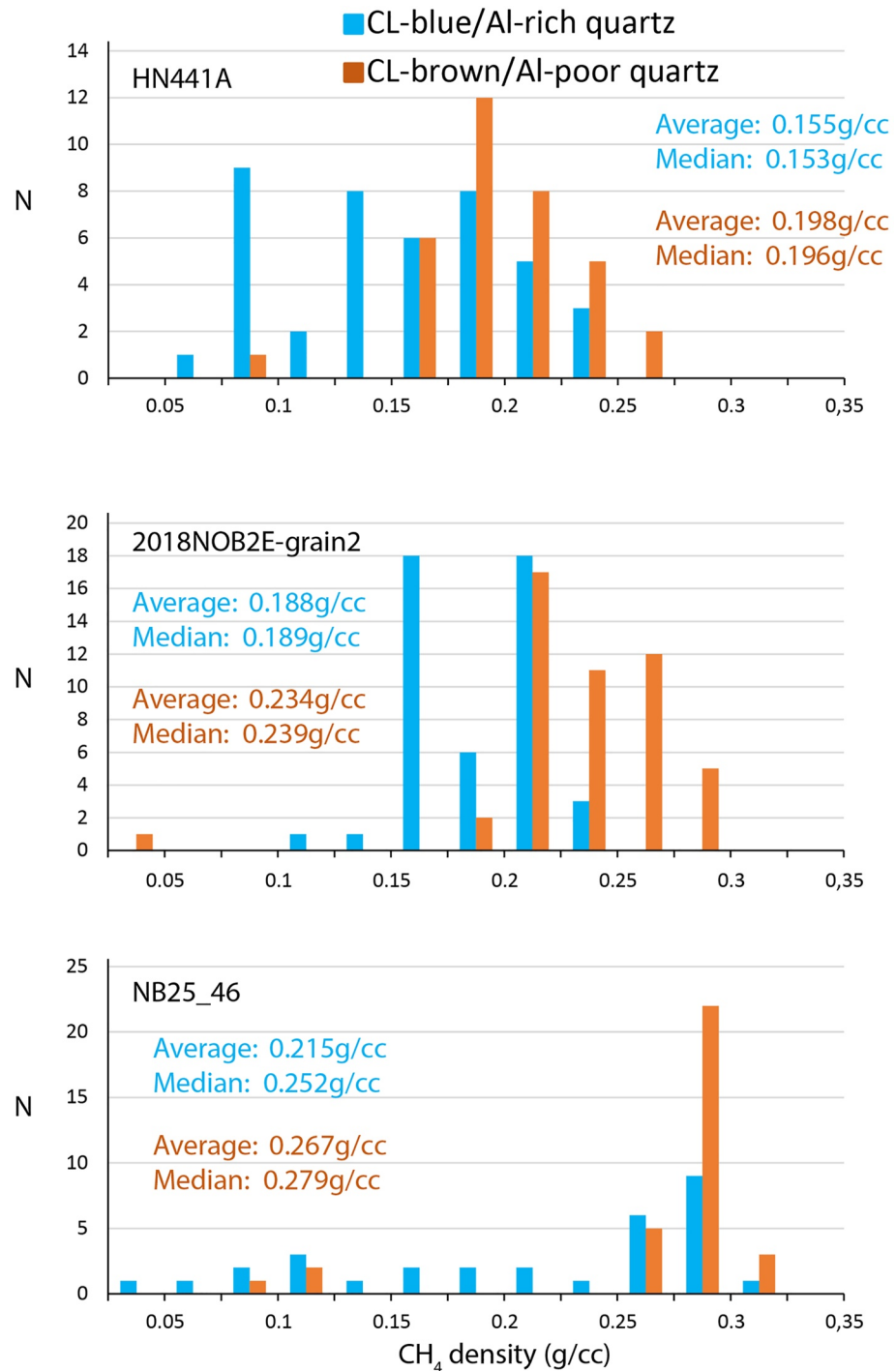
Figure 2. Density histogram of the methane contained in methane-rich fluid inclusions, with a coloring that depends on the cathodoluminescence (CL)-brown or CL-blue domain of host quartz the inclusions belong to. The methane-filled fluid inclusions measured are shown as outlines in Figure 1.
