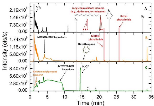
Figure 11. Gas chromatograms recorded after the Sample Analysis at Mars (SAM)-like pyrolysis ( 40^{\circ}\text{C} – 850^{\circ}\text{C} at a 35^{\circ}\text{C}\cdot\text{min}^{-1} rate) of valine in jarosite (a) as is, (b) in the presence of 1 wt% calcium perchlorate and, (c) in the presence of both 1 wt% calcium perchlorate and MTBSTFA-DMF in black, orange, and green respectively. *Derivatized molecules. MTBSTFA-DMF byproducts include monosilylated water, trifluoromethylacetamide (TFMA), DMF (unreacted), tert -butyldimethylfluorosilane (b and c), and chloro- tert -butyldimethylsilane (b).
