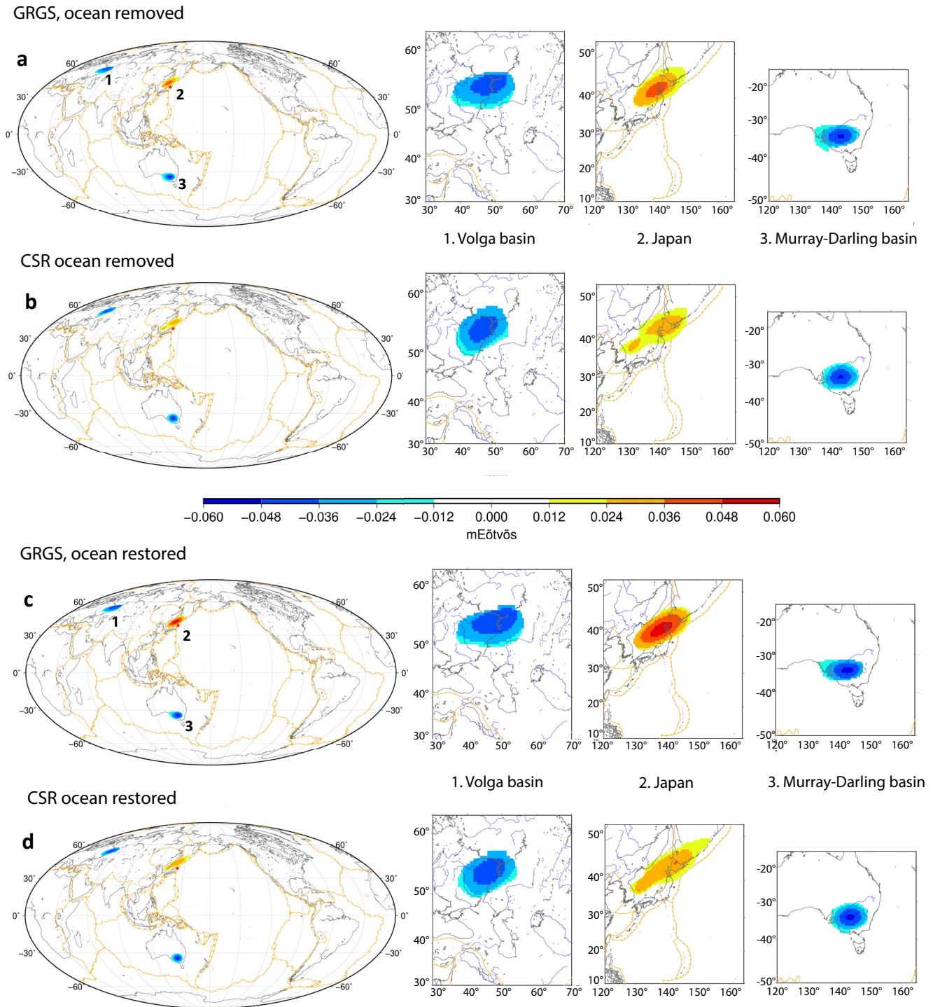
Figure 8. Most consistent signals in the degraded GRGS and CSR solutions in February 2011. Same as Figure 7, for a lower level of sensitivity to both the ocean dealiasing model and the GRACE solution and for all gravity models, with or without restoration of the ocean model (GRGS solutions in (a, c) |k| \leq 0.34 ; S \geq 0.8 ; CSR solutions in (b, d) |k| \leq 0.42 ; S \geq 0.8 ). Zooms in the areas of the three remaining signals (Volga and Murray-Darling drainage basins, Japan Sea) are shown in the right inset maps.
