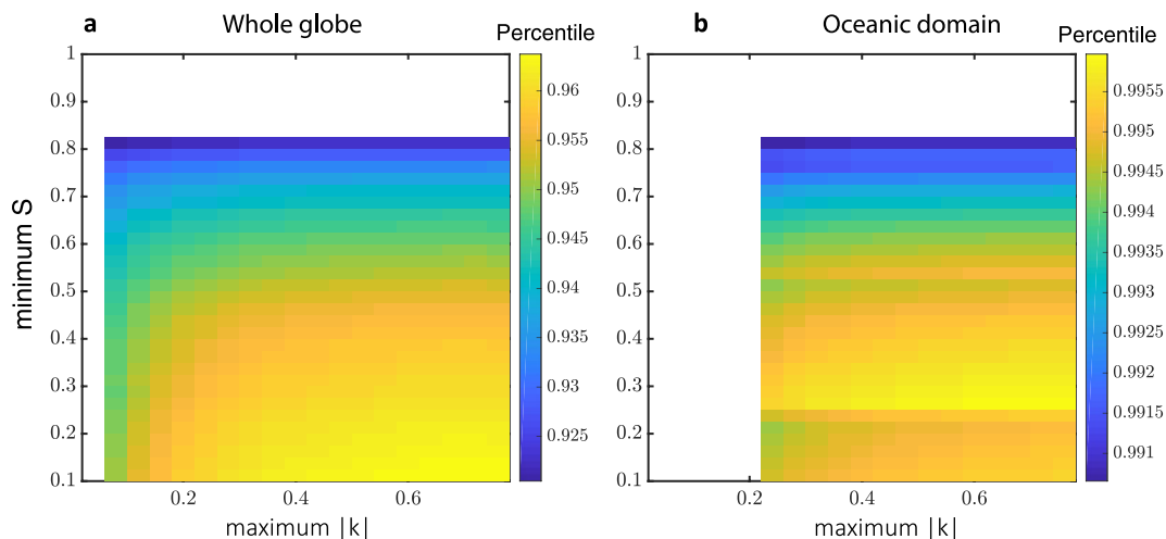
Figure C2. Same as Main Figure 6c and 6f, for the negative lobe of the February 2011 Tohoku preseismic anomaly.
