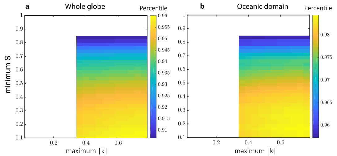
Figure C3. Same as Main Figure 10b and 10c, for the degraded GRGS solution (dealiasing ocean model removed).
