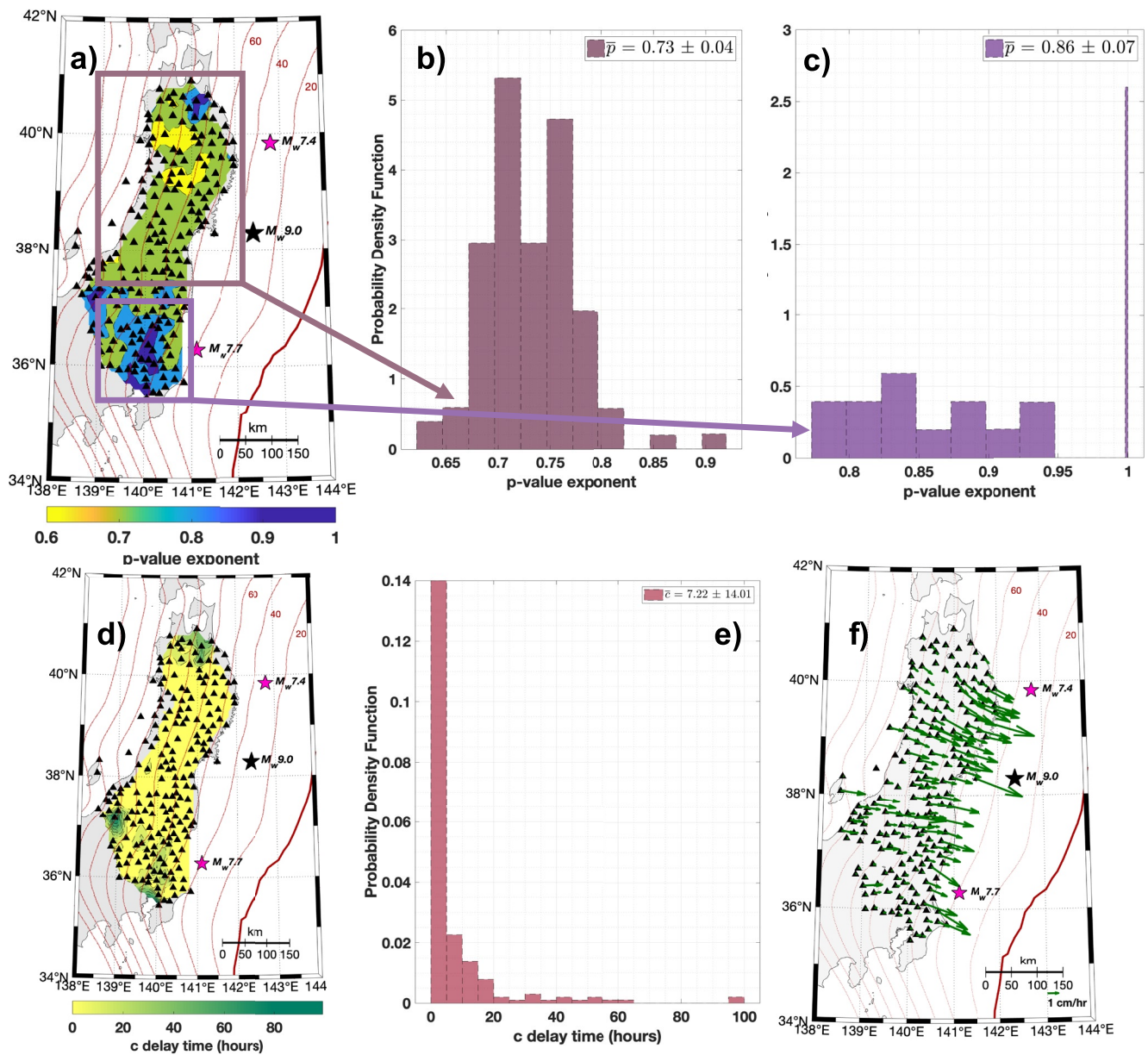
Figure 4. Parameters and statistics obtained on 203 stations successfully inverted for time series up to 1 month: p -value exponents (a) Interpolated map and (b) Statistics and distribution of North area (c) Statistics and distribution of South area. Time delay c in hours (d) Interpolated map and (e) Statistics. (f) Map of horizontal initial velocity v_0 .
