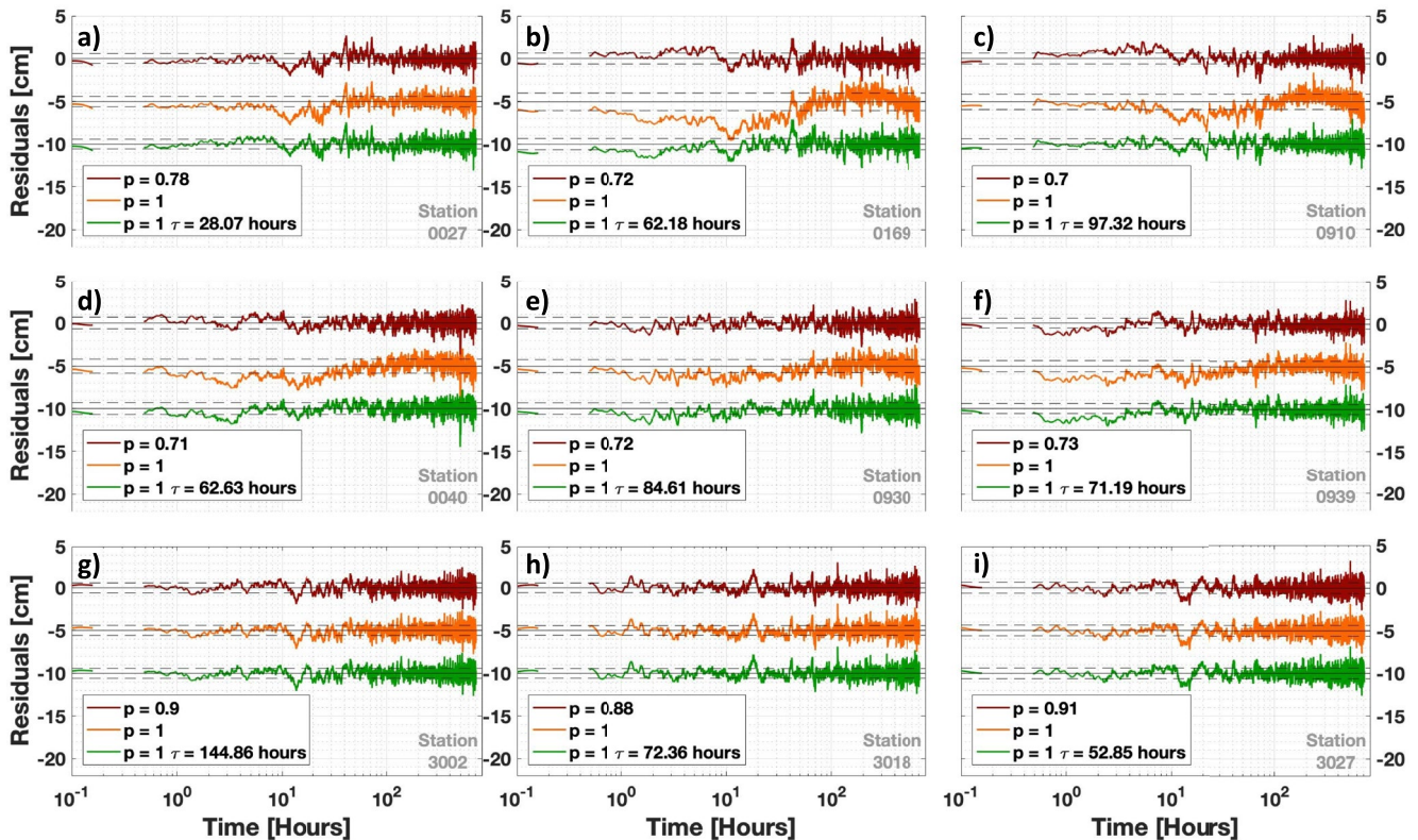
Figure 3. Residuals Analysis. (a–i) Residual displacements on the East component during the first month after the mainshock in logarithmic scale on the x -axis, for three models: The transient brittle creep mechanism described by an “Omori-like” signature characterized by a p -value < 1 (Equation 10—red curves), the velocity-strengthening afterslip associated to a 1/t decay of the velocity (Equation 7—orange curves) and the combination of mantle viscoelasticity and velocity-strengthening afterslip (Equation 11—green curves). The purely viscoelastic model (Equations 2 and 4—blue curve in Figure 2) is excluded because it fits the data poorly. Station locations are represented on Figure 1b (gray triangles) and situated (a–c). Near the coast of Tohoku (d–f). Center of Japan (g–i). Near the coast of Ibaraki.
