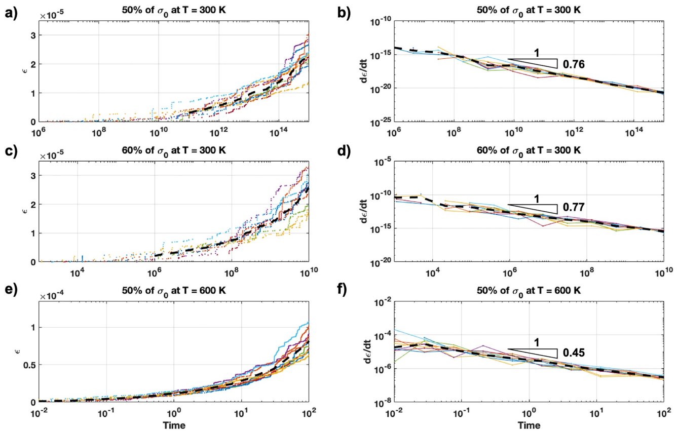
Figure 12. Strain \epsilon (left) and Strain Rate d\epsilon/dt (right) obtained for the creep deformation of the modeled domain, with the following modeling parameters: Friction coefficient \mu = 0.7 , constant loading maintained at 50% or 60% of the stress remaining after the stress drop of the pre-loading stage, for T = 300 K (a–d) or T = 600 K (e–f). Ten simulations corresponding to different realizations of the initial disorder were performed in each case, and the black dotted curves represent the average response where the slopes represent the p -values estimated. The present curves focus on the transient creep (stage I).
