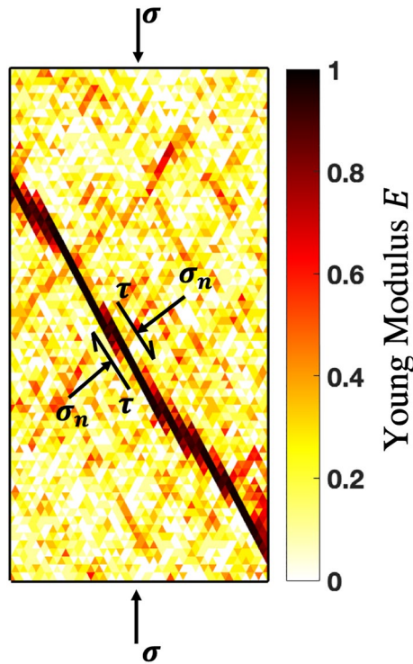
Figure 11. Progressive damage modeling of transient brittle creep. The elastic domain is discretized into N -finite elements of initially equal Young's modulus E_0 but a variable cohesion. The figure represents the damage field obtained at the end of the athermal pre-loading stage, with an incipient inclined fault. The color represent the damage values, normalized such that the maximum damage values, that is, the minimum elastic moduli, are shown in black along the fault. This faulted domain is then reloaded under a constant external uniaxial creep stress \sigma , with thermal activation switched on. This leads to a resolved shear stress \tau along the fault plane and a normal stress \sigma_n .
