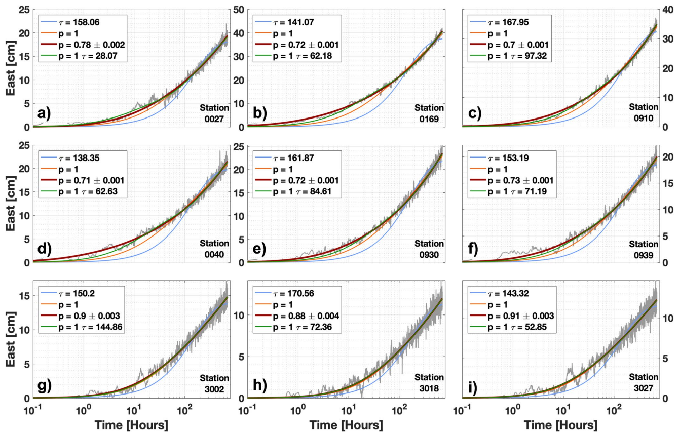
Figure 2. Temporal Evolution and models used to fit GPS kinematic time series. (a–i) Displacement evolution on the East component (gray curve) during the first month after the mainshock in logarithmic scale on the x -axis. Different mechanisms and models are tested, the viscoelastic model with an exponential velocity decay (Equation 2 or Equation 4—blue curves), the velocity-strengthening afterslip associated with a logarithmic increase of the displacement (Equation 7—orange curves), the transient brittle creep mechanism described by an “Omori-like” signature characterized by a p -value (Equation 10—red curves) and the combination of mantle viscoelasticity and velocity-strengthening afterslip (Equation 11—green curves). Station locations are represented on Figure 1b (gray triangles) and situated (a–c). Near the coast of Tohoku (d–f). Center of Japan (g–i). Near the coast of Ibaraki.
