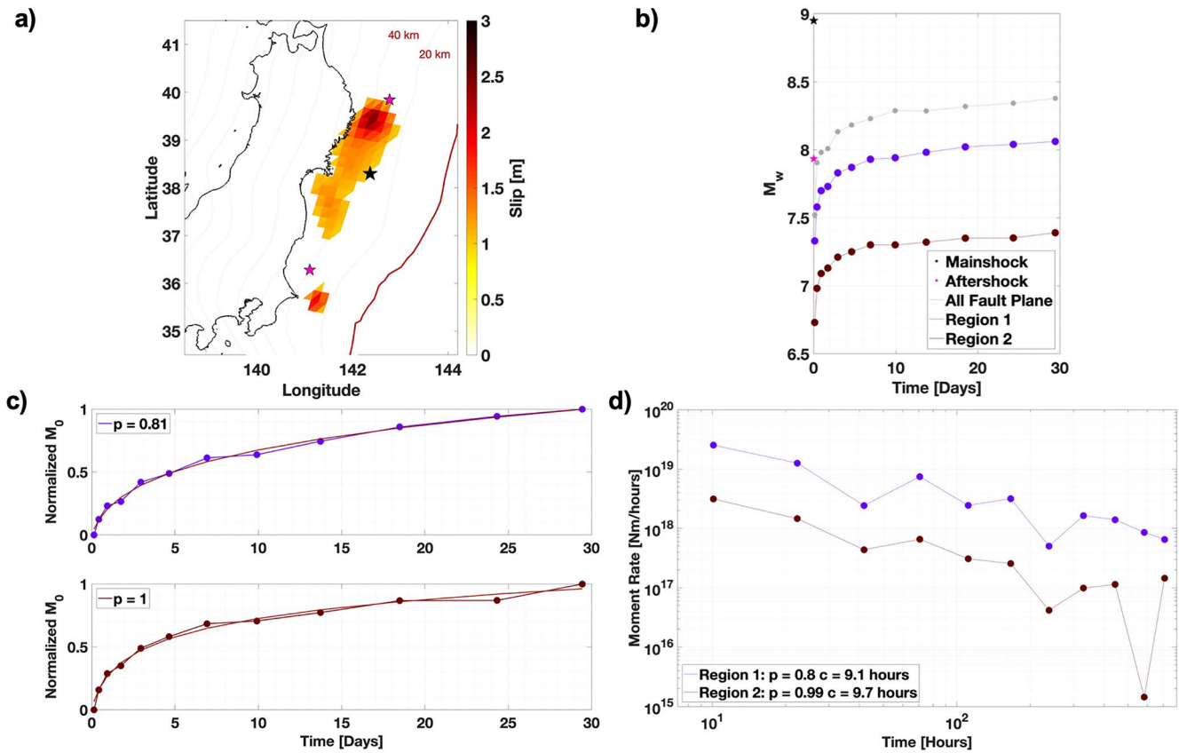
Figure 10. (a) Afterslip during the first month following Tohoku-Oki divided in two main areas: region 1 in the North (afterslip central and northern patch near the Iwate-Miyagi coast) and region 2 in the South (afterslip near Ibaraki coast) are defined by a slip larger than 1 m (b) Equivalent seismic magnitude of the postseismic slip computed over time for all the fault plane (gray line), region 1 (blue line) and region 2 (brown line). Black and magenta stars represent the seismic magnitudes of the mainshock and the aftershock, respectively. (c) Equivalent seismic moment normalized between 0 and 1 over time, black lines represent the best-fit following Equation 10 for both regions. (d) Moment Rate computed over the time window ( t_0^* + 10.1 hr and t_0^* + 29.4 days).
