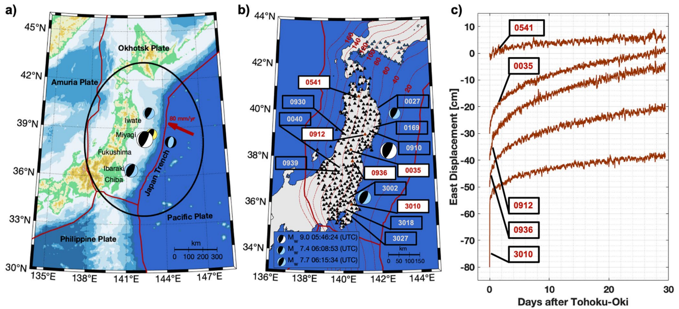
Figure 1. Maps of the Japan Area and examples of GPS kinematic time series. (a) Plate boundaries are illustrated in red, the associated Pacific interseismic loading ( \sim 80 mm/year) is represented with the red arrow. Significant earthquake focal mechanisms (F-net catalog) sorted by size (yellow as foreshock, black as mainshock, black and blue as largest aftershocks). Stations used for this study are located within the black circle (distance from the mainshock epicenter less than 500 km). (b) Black triangles are stations used for this study, brown triangles illustrate stations shown on Figure 1c, gray triangles are stations represented on Figures 2, 3, 5 and 6 and blue triangles are stations used to build the stack for the common modes correction. Earthquakes recorded by our kinematic data are the mainshock as well as the Ibaraki-Oki and largest north aftershock. Plates boundaries (red lines) and isodensity of the fault are given (thin red lines). (c) Postseismic signal from five different stations (shown on Figure 1b) on East component after the kinematic processing and post-processing phases applied (Sidereal Filtering and Removing Common Modes).
