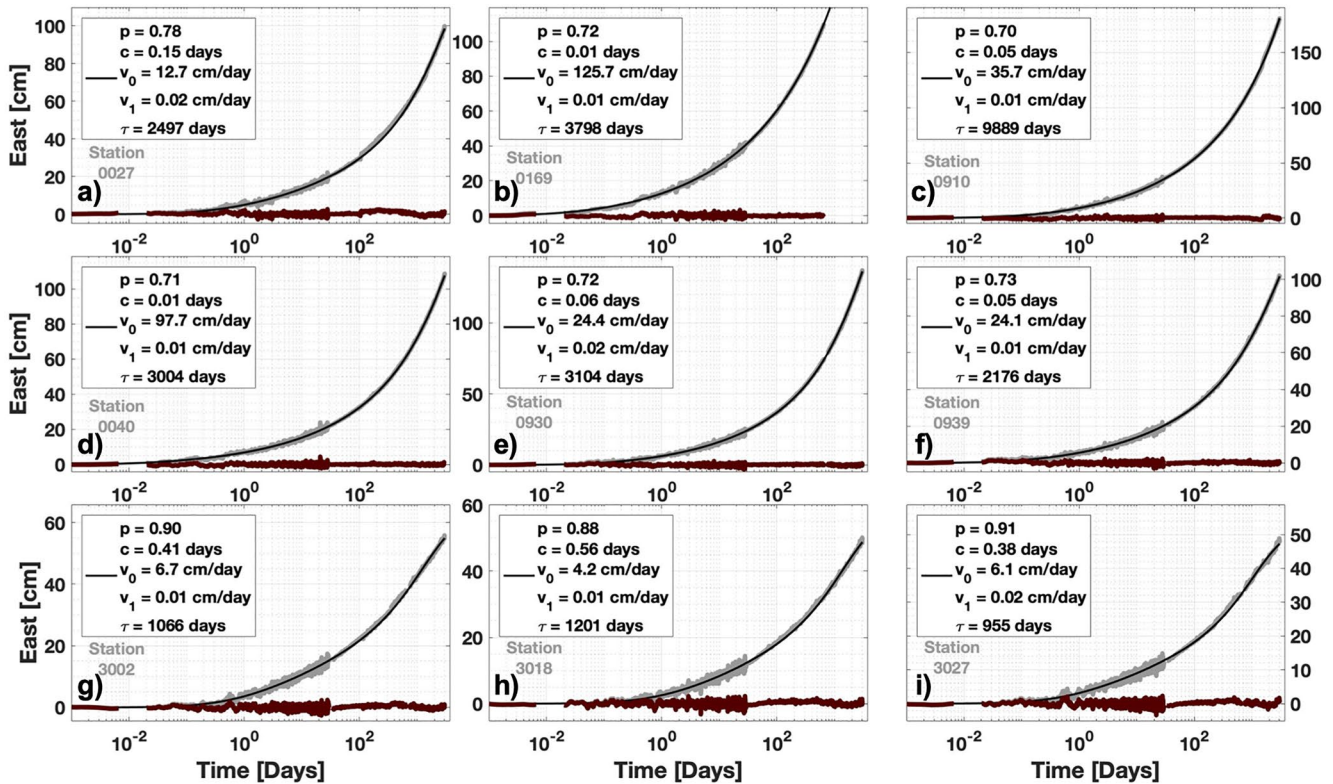
Figure 6. Temporal Evolution and models used to fit GPS kinematic + static time series up to \sim 2020 . (a–i) Displacement evolution on the East component (gray) during \sim 9 years after the mainshock in logarithmic scale on the x -axis. The transient brittle creep mechanism determined by a p -value is combined with an exponential decay function associated with a mantle viscoelastic mechanism (Equation 2 or Equation 4) which the nature is debated in the discussion (black curves). Final residual displacements (brown curves). Station locations are represented on Figure 1b (gray triangles) and situated (a–c). Near the coast of Tohoku (d–f). Center of Japan (g–i). Near the coast of Ibaraki.
