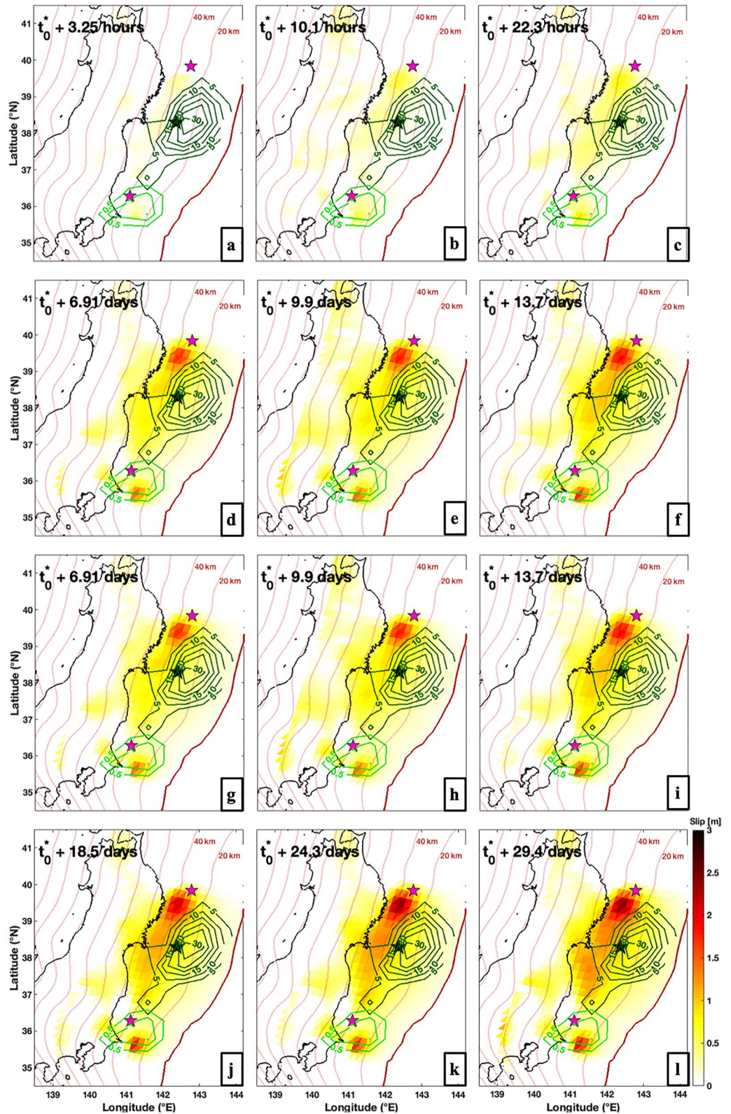
Figure 9. Spatio-temporal evolution of afterslip during the first month on 12-time windows: Afterslip(s) coseismic offsets are removed from the postseismic deformation. Green lines represent slip contours of the Tohoku-Oki mainshock and Ibaraki-Oki aftershock in meters. Stars correspond to the three main events. Color scale indicates the slip amplitude in meters.
