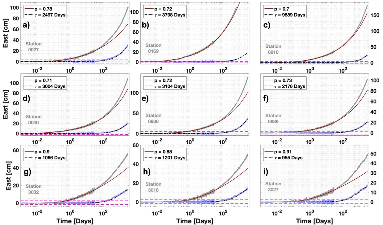
Figure 5. Residuals Analysis of transient brittle creep model on the combination of GPS kinematic (over 1 month), + static time series up to ~2020. (a–i) Displacement evolution on the East component (gray curve) during ~9 years after the mainshock in logarithmic scale on the x -axis. The p -value of the transient brittle creep (Equation 10—red curves) was determined over the first month. Then, the related residuals displacements are computed (blue curves) over large timescales. The black dashed-dotted curves correspond to Equation 2 or Equation 4. RMS of residual displacements is shown (magenta dotted lines). Stations locations are represented on Figure 1b (gray triangles) and situated (a–c). Near the coast of Tohoku (d–f). Center of Japan (g–i). Near the coast of Ibaraki.
