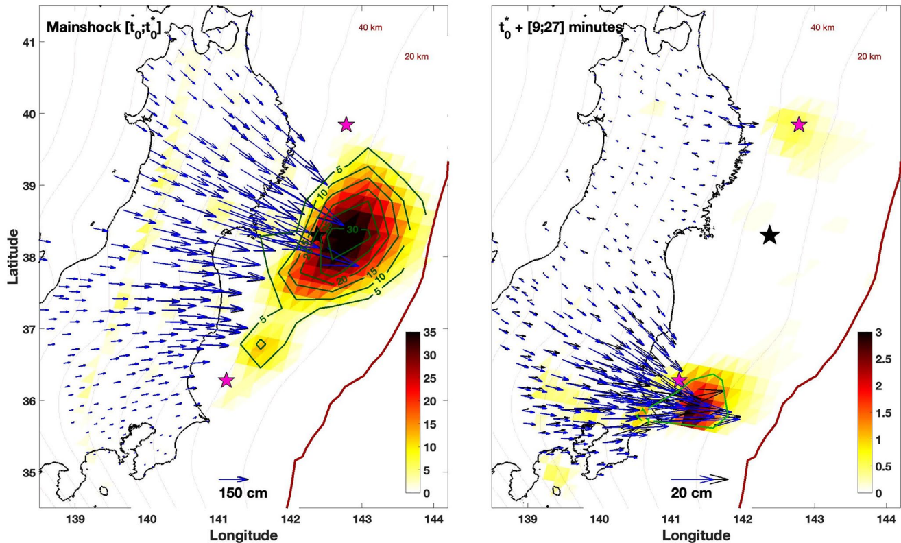
Figure 8. Spatio-temporal evolution of (a). Tohoku-Oki coseismic offset (05:46:00–05:56:00 UTC) with \chi^2 = 16.2 (b). Ibaraki-Oki coseismic offset (06:06:00–06:24:00 UTC) with \chi^2 = 2.8 . Black and blue arrows represent observed and predicted horizontal displacements. Green lines represent slip contour in meters. Stars correspond to the epicenters of the three main events. Color scale indicates the slip amplitude in meters.
