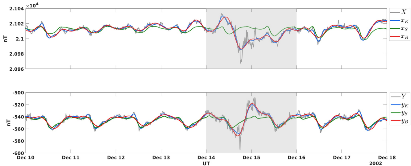
Figure 9. Comparison of baseline methods. The methods of the introduced baseline (red), Finnish Meteorological Institute (blue) and SuperMAG (green) for X, Y components (grey) at Chambon-la-Forêt during winter 2002 are presented. The grey shaded areas indicate non-CK48 days.
