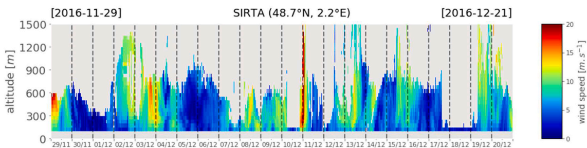
Fig. 5. Time series of vertical profile of horizontal wind speed measured by the WLS70 Doppler lidar installed at Sirta observatory between November 29, 2016, and December 21, 2016.
