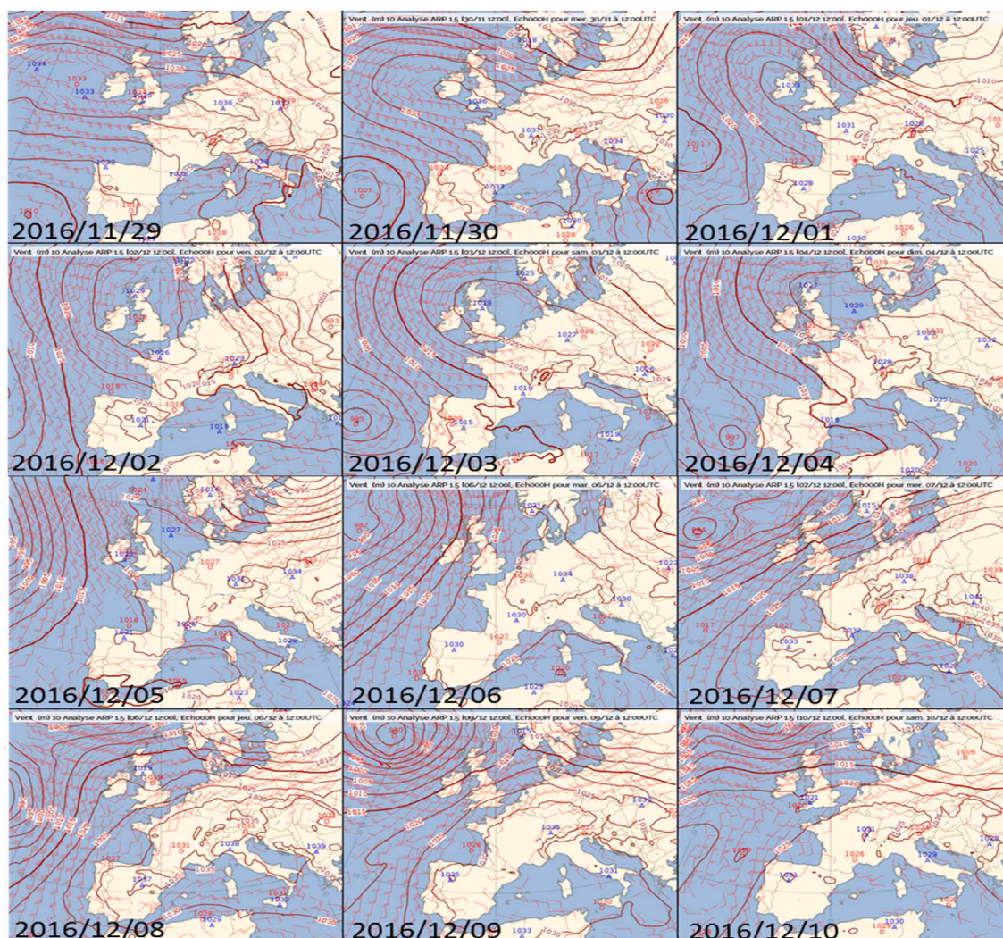
Fig. 4. Surface pressure and 10 m winds from ARPEGE analysis for the period ranging between November 29th and December 10th, 2016 (Source Météo-France).
