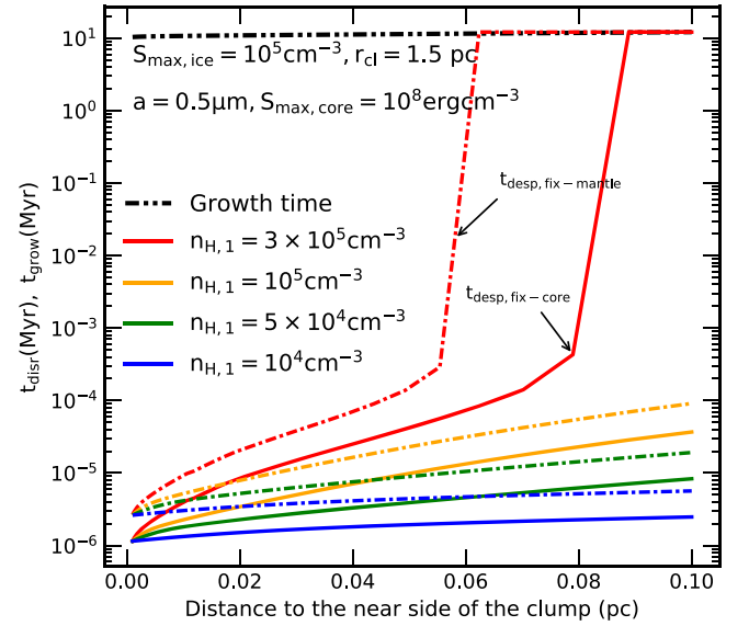
Figure 14. Variation of rotational desorption timescales for icy grain mantle of size a = 0.5 \mu\text{m} inside a clump at r = 1.5 pc with different gas density profiles, for ice mantles with S_{\text{max,ice}} = 10^7 \text{ erg cm}^{-3} (upper panel) and S_{\text{max,ice}} = 10^5 \text{ erg cm}^{-3} (lower panel), respectively. A comparison between the removal of ice mantles on a fixed grain core of a_c = 0.08 \mu\text{m} (solid lines) and a fixed ice mantle thickness of \Delta a_m = 0.05 \mu\text{m} (dashed-dot lines) is also presented.
