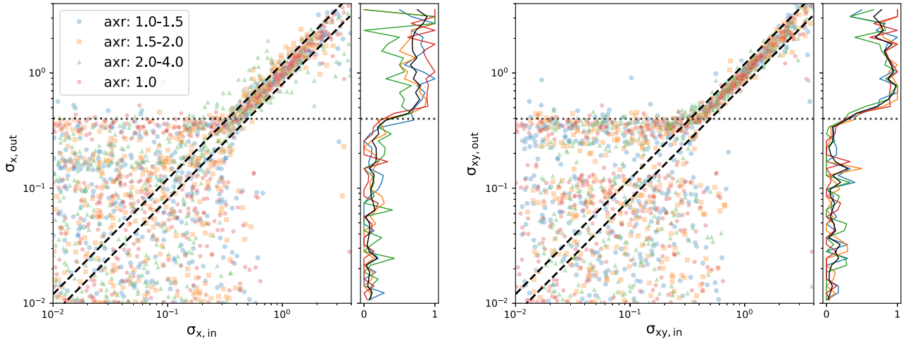
Figure C1. Standard deviation resulting from the fit of synthetic sources in function of their input values. Left-hand panel shows \sigma for the minor axis ( \sigma_x ), right-hand panel shows the geometrical mean \sigma_{xy} \equiv \sqrt{\sigma_x \cdot \sigma_y} . Different colours and symbols refer to sources with different axis ratios, as reported in the legend. The dashed lines enclose the good fits, i.e. where the relative error on the retrieved size is less than 20 per cent. The horizontal dotted line mark the \sigma_{x,\min} = 0.4 pixels value chosen as the minimum resolvable size. For each panel, the subpanel on the side shows the fraction of sources with good fit in function of the output standard deviation.
