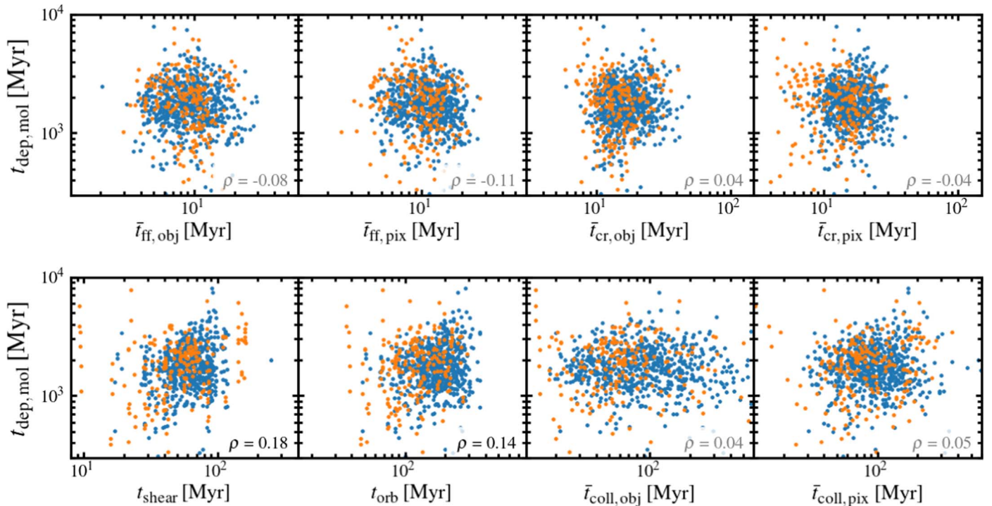
Figure 8. Correlations between molecular gas depletion time ( t_{\text{dep,mol}} ) vs. each of the other timescales shown in Figure 7. The x-axes of all panels are scaled to show the same logarithmic range. Measurements in the “disk” and “center/bar” samples are denoted by data points in blue and orange, respectively. We display Spearman’s rank correlation coefficient for all measurements at the lower-right corner in each panel, with black (gray) font color indicating a p -value smaller (larger) than 0.001.
