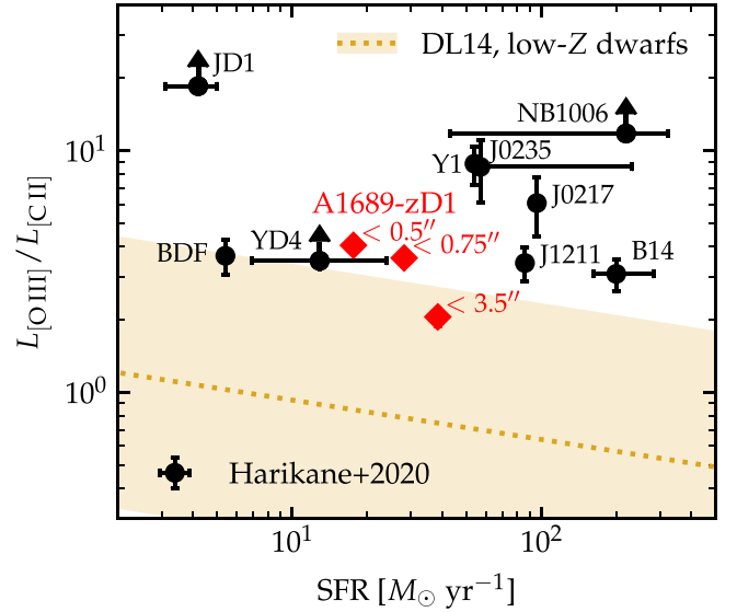
Figure 11. The L_{[\text{O III}]} / L_{[\text{C II}]} ratio vs. SFR for A1689-zD1 in multiple apertures (red diamonds), compared to the literature sample from Harikane et al. (2020) (black circles). The SFR values are computed as described in Section 3.4. While the L_{[\text{O III}]} / L_{[\text{C II}]} ratio is lowered by a factor of \sim 2 by accounting for the full [C II] halo, this cannot account for the entirety of the high L_{[\text{O III}]} / L_{[\text{C II}]} ratios in high-redshift galaxies.
