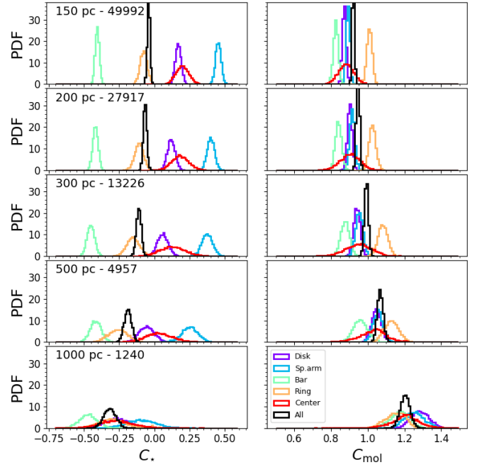
Fig. 6. Posterior distribution of the coefficients that define the star-forming planes in each galactic environment, at each one of the spatial scales probed, from 150 pc to 1 kpc. The spatial scale and the number of pixels used for each measurement are indicated in the top left corner for each row.
