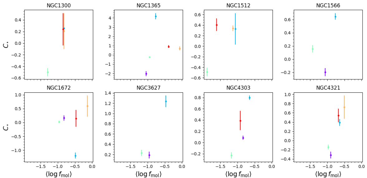
Fig. D.2. C_{\star}-\langle f_{\text{mol}}\rangle correlation across different galactic environments, for the galaxies that satisfy our single-galaxy selection criteria. The color code for each environment is the same as used in Fig. 1.
