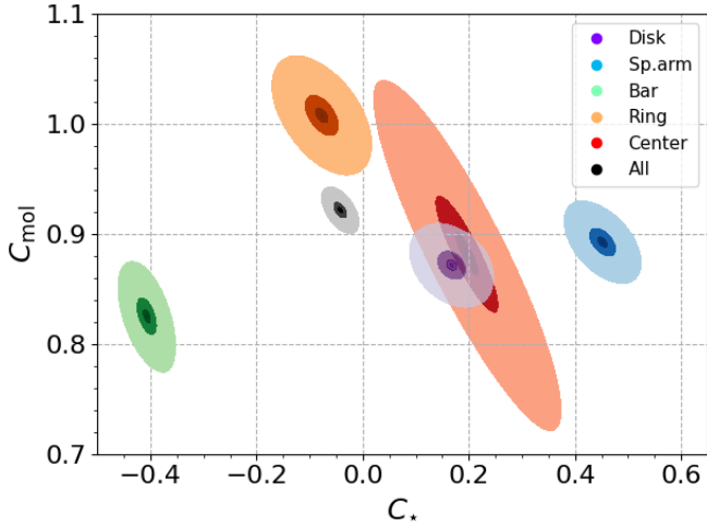
Fig. 3. Posteriors distributions of the coefficients C_* and C_{\text{mol}} for each separate environment, measured at an spatial resolution of 150 pc, to show the covariance between them. The posteriors have been smoothed using a Gaussian kernel. The color scale for each environment indicates the 1-, 2- and 3-sigma confidence intervals.
