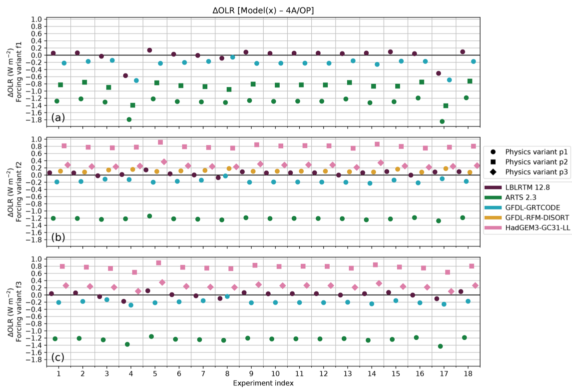
Figure A1. Means and standard deviations of OLR differences (model minus 4A/OP; \text{W m}^{-2} ) as a function of the experiment index. The five models compared to 4A/OP are represented by colors. The three forcing indices f1, f2, and f3 are respectively represented in individual panels (a–c). The different physics variants are differentiated with marker shapes.
