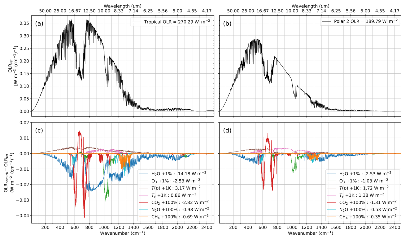
Figure 5. Spectral OLR at a spectral resolution of 1 cm -1 computed for the TIGR mean Tropical atmosphere (a) and TIGR mean Polar 2 atmosphere (b). Corresponding OLR values spectrally integrated between 10 and 2500 cm -1 are provided in the legends. Spectral OLR sensitivity to temperature and composition change for the TIGR mean Tropical (c) and mean Polar 2 (d) atmospheres. Results are expressed as [OLR perturb - OLR ref ] as a function of the wavenumber. The spectrally integrated sensitivities are specified in the legends and in Table 5.
