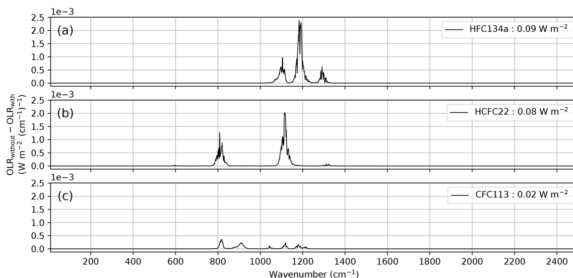
Figure 6. Spectral OLR variation due to a complete removal of atmospheric HFC134a (a), HCFC22 (b), and CFC113 (c) calculated from the TIGR mean Tropical atmosphere. The total longwave OLR variations are reported in the legends. Note that the y axis ranges from 0 to 2.5 \times 10^{-3} \text{ W m}^{-2} (\text{cm}^{-1})^{-1} .
