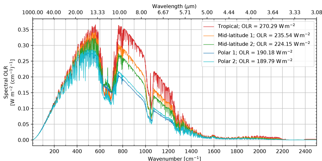
Figure 4. Spectral OLR at a resolution of 1 cm^{-1} computed for the mean atmosphere of each of the five classes of TIGR. Spectrally integrated OLR values in the 10–2500 cm^{-1} range are displayed in the legend.
