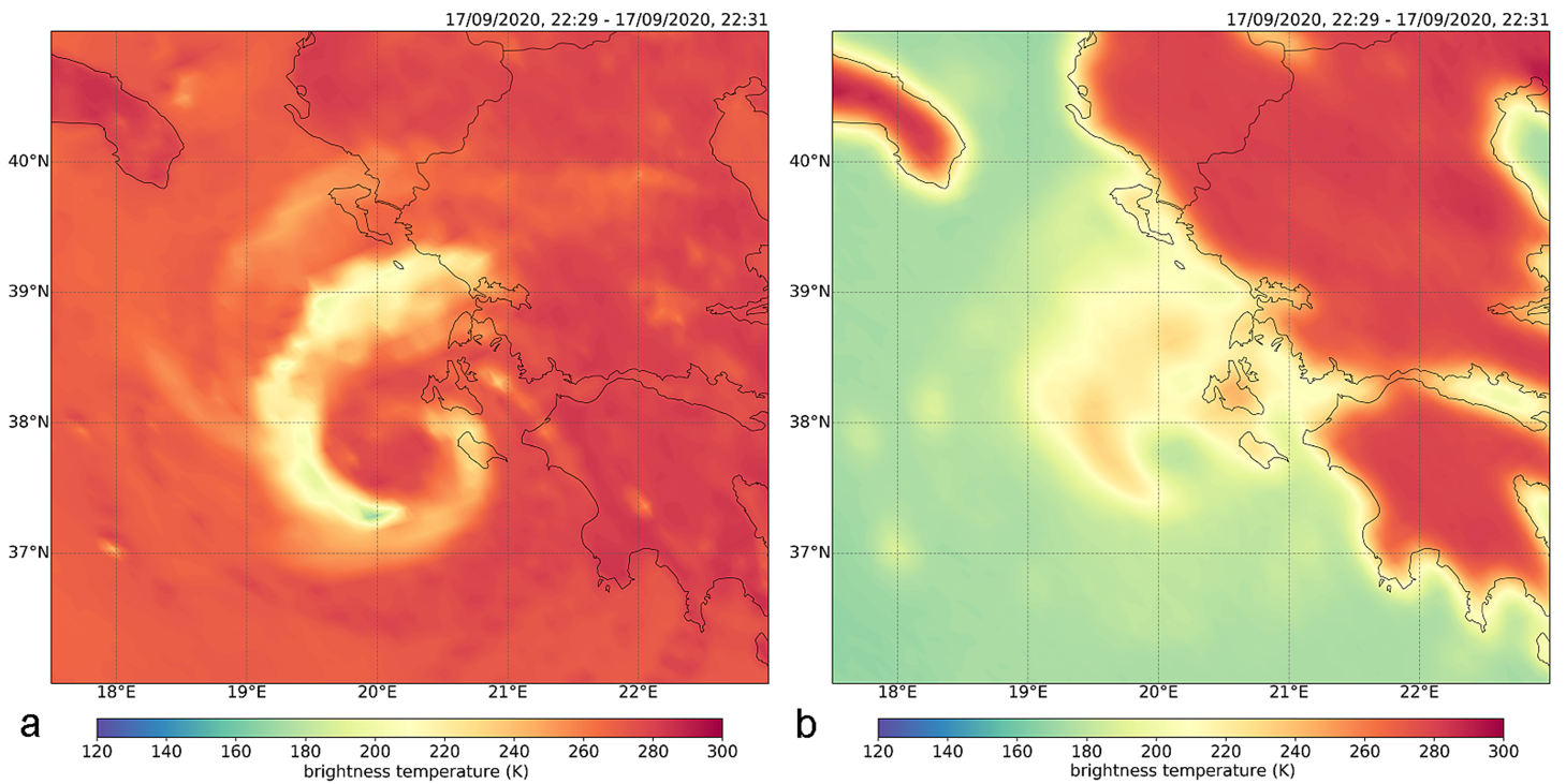
Fig. 10. GPM GMI brightness temperature (K) measured at (a) V89 GHz and (b) V10 GHz around 2230 UTC 17 Sep 2020.
