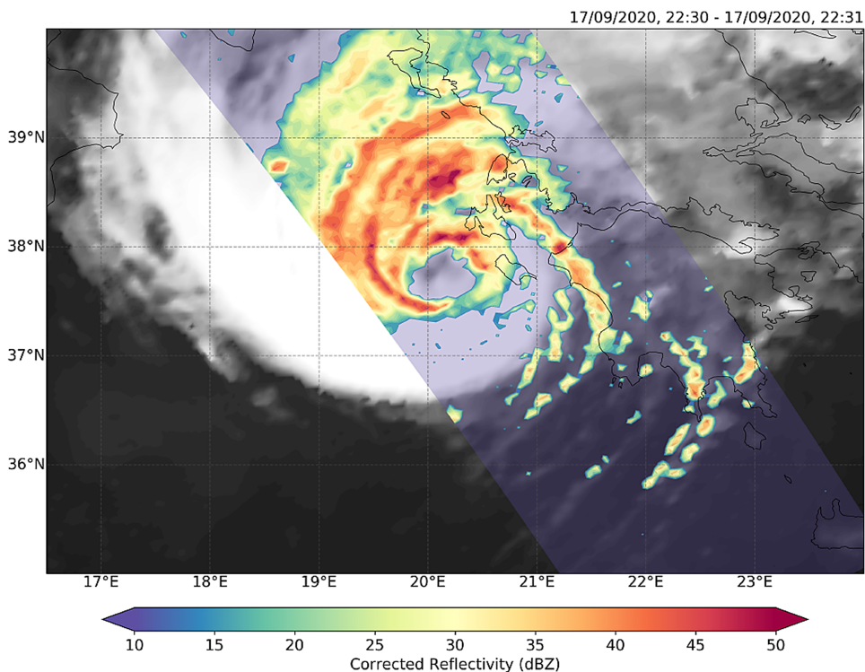
Fig. 11. GPM DPR near-surface corrected reflectivity (normal scan) around 2230 UTC 17 Sep 2020.
