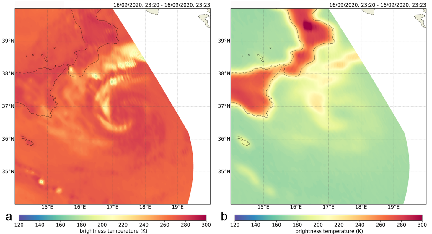
Fig. 9. GPM GMI brightness temperature (K) measured at (a) V89 GHz and (b) V10 GHz around 2320 UTC 16 Sep 2020.
