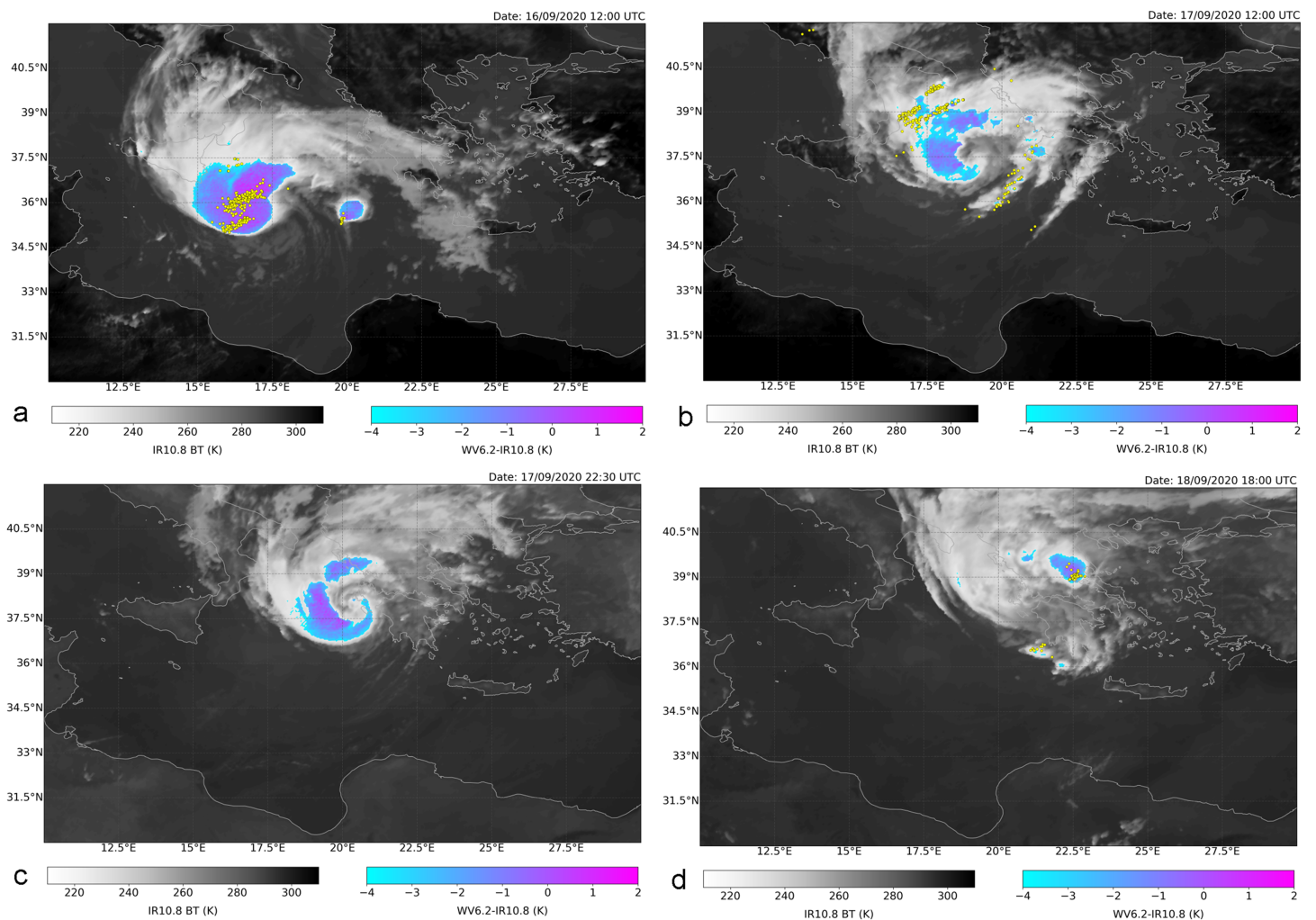
Fig. 4. MSG SEVIRI infrared brightness temperature (grayscale), and brightness temperature difference between the WV6.2 and IR10.8 channels (color scale), valid at (a) 1200 UTC 16 Sep, (b) 1200 UTC 17 Sep, (c) 2230 UTC 17 Sep, and (d) 1800 UTC 18 Sep 2020. Yellow dots denote lightning strikes detected by ZEUS network within 60 min before and after the satellite nominal time.
