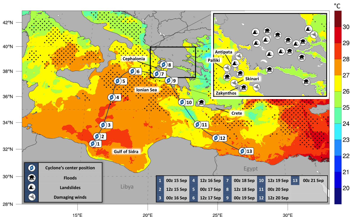
Fig. 1. Path of Medicanes Ianos, from 0000 UTC 15 Sep up to 0000 UTC 21 Sep 2020. Shading denotes the SST (at 1-K intervals), and the black dots the daily SST anomaly higher than 2 K on 15 Sep 2020. Symbols for floods, landslides, and damaging winds are placed over the most affected areas.
