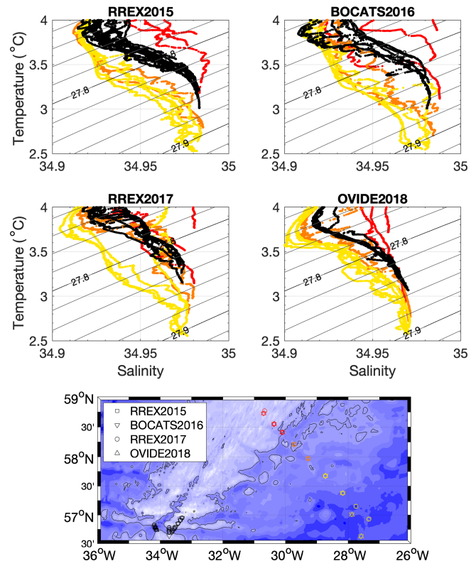
Figure 3. \theta – S diagram of the (color) southward along-ridge flow and (black) westward cross-ridge flow through the BFZ for each cruise indicated in the lower panel. The black line outlines the 2100 m isobath.
