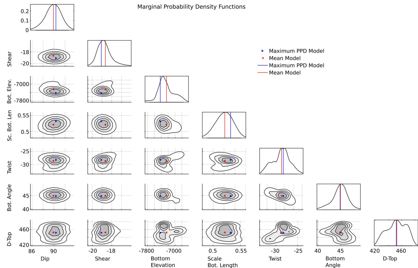
Extended Data Fig. 6 | Inversion results. One-dimensional (diagonals) and two-dimensional (off-diagonals) marginals posterior probability density functions.
