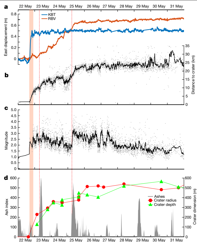
Fig. 2 | Time series of co- and post-eruptive signals. a , Eastward displacement recorded at KBT (blue) and RBV (orange) GNSS stations. b , Distance to crater (km) of automatically located earthquakes (grey dots) overlaid with a 15-event moving average (black line). c , Magnitude of earthquakes (grey dots) overlaid with a 15-event moving average (black line). d , Volcanic ash index (from SEVIRI InfraRed satellite) and crater dimensions from SAR imagery analysis. Crater depth is estimated with reference to the 2002 platform at around 3,190 m (Methods). The around 6 h effusive activity and main ash column emission at the summit (23 and 25 May) are marked by the red shading and dotted lines, respectively.
