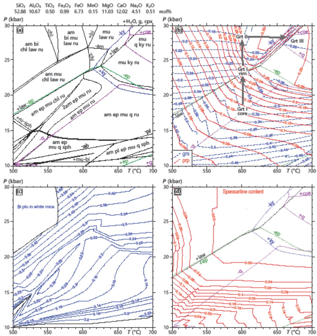
Figure 6. P–T pseudosections for eclogite sample NO7A calculated for the indicated bulk composition (H 2 O is considered in excess). Some small fields are unlabelled for clarity. Grey arrows indicate the inferred P–T path. Kyanite, quartz/coesite, epidote and lawsonite stability fields reported in (b) and (d) as in (a). See text for further details.
