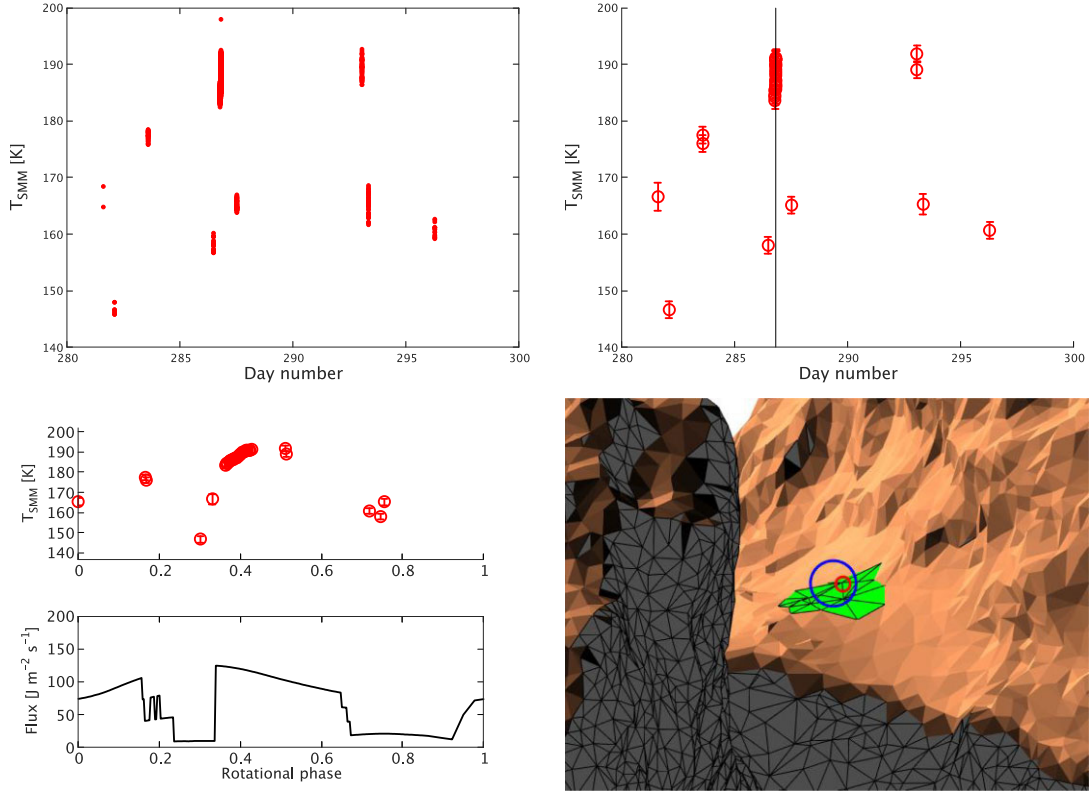
Figure 6. Upper left-hand panel: Raw SMM 1-s continuum MIRO antenna temperature observations of Hapi D in October 2014, on the original time-line, assuming a beam efficiency (see text) of B_e = 0.96 . Upper right-hand panel: Binning the SMM data into 2.4 min-wide bins (error bars show the standard deviation for the data within a given bin), on the original time-line. Middle left-hand panel: The binned SMM data are here time-shifted to a common master period. Lower left-hand panel: The time-shifted data are here compared to the flux (direct solar illumination plus infrared self-heating) as described in Section 3.1. Lower right-hand panel: The nucleus of 67P as seen from the Rosetta spacecraft on 2014 October 13, at 19 : 21 UTC, during the continuous stare. The intensity of the copper colour scales with the local solar flux, grey areas are in shadow, the green field shows Hapi D, and the red (SMM) and blue (MM) rings are the MIRO FWHM beam footprints.
