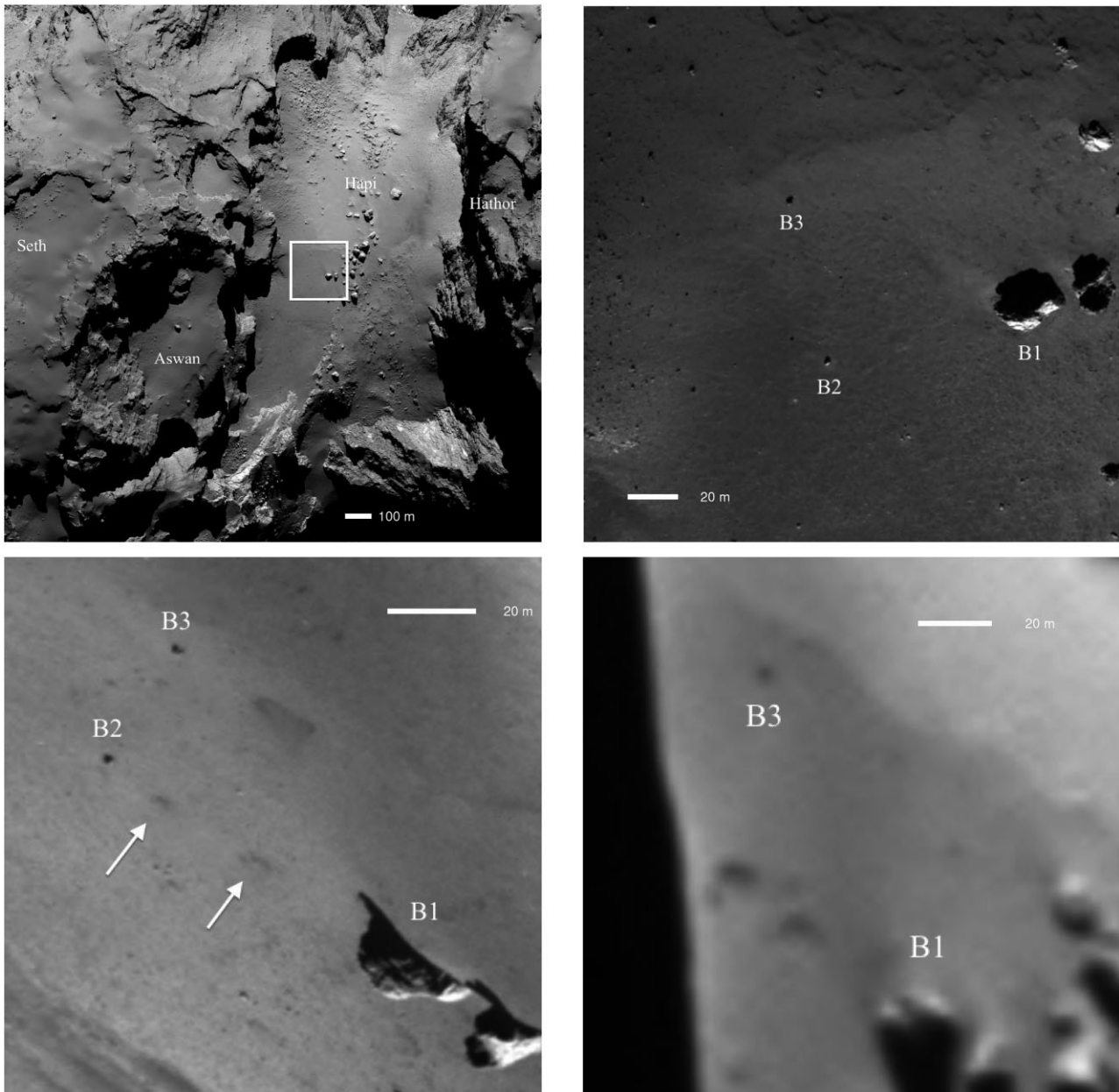
Figure 1. Upper left-hand panel: NAC context image of Hapi and surroundings taken on 2014 August 30. The large lobe is to the left and the small lobe is to the right (outside the image). The distance from Rosetta to the comet surface was approximately 55.5 km and the resolution was 0.98 \text{ m px}^{-1} . The square marks the area in which the currently discussed changes took place, and is the approximate field of view in the upper right panel. Image MTP006/n20140830t034253546id20f22.img. Upper right-hand panel: This NAC image of a small portion of the Hapi region was acquired on 2014 December 10, prior to any detectable change (see the upper left-hand panel for context). The distance from Rosetta to the comet surface was \sim 19.9 \text{ km} and the resolution was 0.35 \text{ m px}^{-1} . The boulder B1 measures 27.4 \pm 0.4 \text{ m} across. Boulders B2 and B3 are 1.8 \pm 0.4 \text{ m} and 2.1 \pm 0.4 \text{ m} across, respectively, and the projected distance between the two is 65.5 \pm 0.4 \text{ m} . Image MTP010/n20141210t062855791id20f22.img. Lower left-hand panel: This NAC image, taken on 2014 December 30, shows the first-known indications of changes (two dark features marked with arrows). The distance from Rosetta to the comet surface was approximately 27.8 km and the resolution was 0.49 \text{ m px}^{-1} . The surface is seen at a high emergence angle that distorts the perspective. The left feature is 4.9 \pm 0.5 \text{ m} across, and the right feature is 7.7 \pm 0.5 \text{ m} across. Image MTP011/n20141230t081300834id20f22.img. Lower right-hand panel: This WAC image was taken on 2015 January 11. The distance from Rosetta to the comet surface was approximately 27.1 km and the resolution was 2.57 \text{ m px}^{-1} . The features have grown with respect to the lower left-hand panel. The left feature is 12.9 \pm 2.6 \text{ m} across, and the right feature is 13.1 \pm 2.6 \text{ m} across. Image MTP011/w20150111t125858091id20f13.img.
