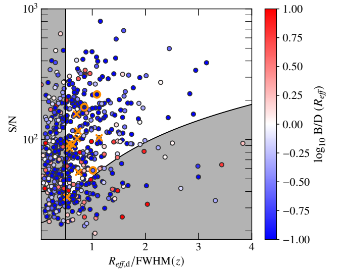
Fig. 9. S/N-disk effective radius-B/D selection plot for galaxies from the kinematics sample. The disk size selection criterion is represented as the vertical line. The S/N selection criterion depends on the FWHM, which varies with redshift and MUSE field. As an example, we show the S/N limit used for a typical FWHM of 0.65'' . Points are colour-coded according to their bulge-to-disk ratio computed at one effective radius. The grey areas give an idea of the galaxies eliminated by the size and S/N selection criteria. We also show the ten galaxies eliminated by selection criterion v (orange crosses) and the three we decided to keep (orange circles).
